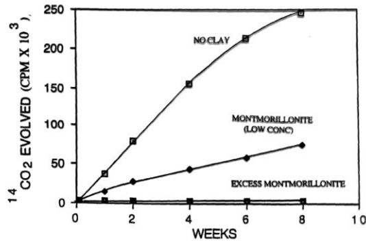
FIG. 8.1 Mineralization of 14 C-labeled diquat in nutrient solutions with or without clay. (Reprinted with permission from Weber and Coble, 1968.)
