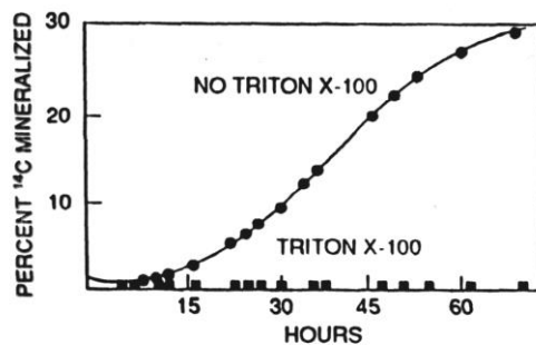
FIG. 9.6 Effect of Triton X-100 on the mineralization by Arthrobacter sp. of hexadecane dissolved in heptamethylnonane. (From Efrøymson and Alexander, 1991. Reprinted with permission from the American Society for Microbiology.)
