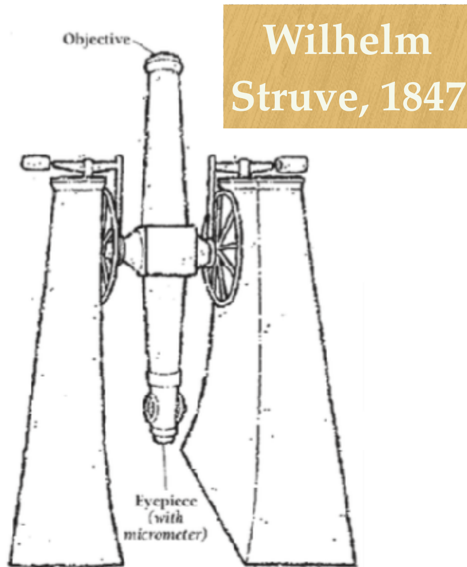
Figure 5.2 The transit telescope. A typical transit telescope is supported between two heavy piers, and can rotate only on one axis to show objects on the observer's meridian. The transit telescope was designed for the measurement of accurate stellar or planetary positions. The angle of elevation of the telescope, and the time at which the object transited the observer's meridian (as seen by the passage of the object across the wire in the micrometer) gave its declination and right ascension. (Credit: Layne Lundström.)
