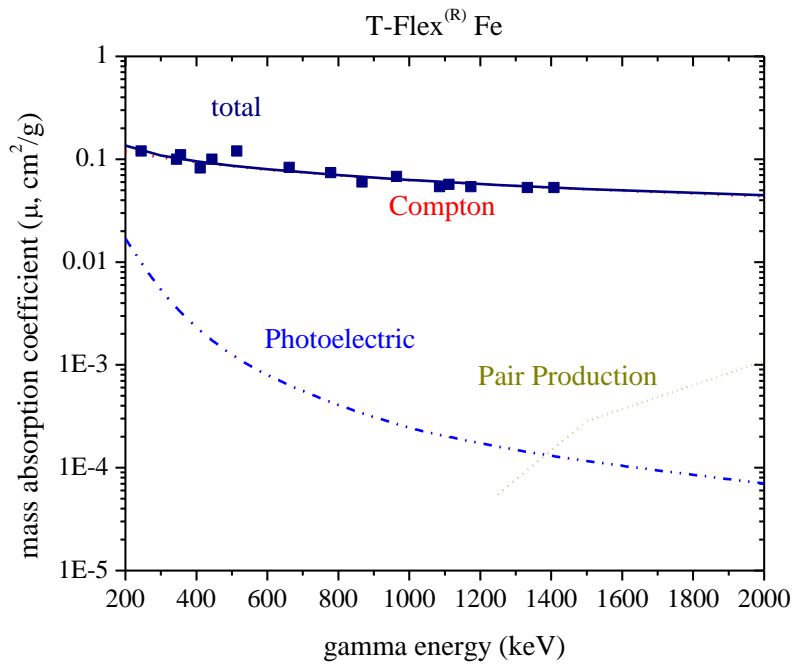
Figure 1d. Attenuation of gamma radiation T-Flex (R) Fe. Measured values (squares). XCOM calculated values (lines)
