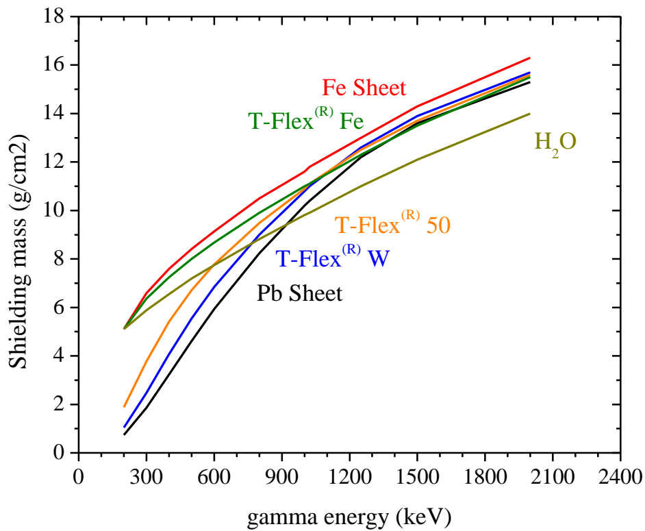
Figure 6. Mass of shielding per surface area ( \text{g/cm}^2 ) required to achieve 50% attenuation versus gamma radiation energy for selected shielding types.
