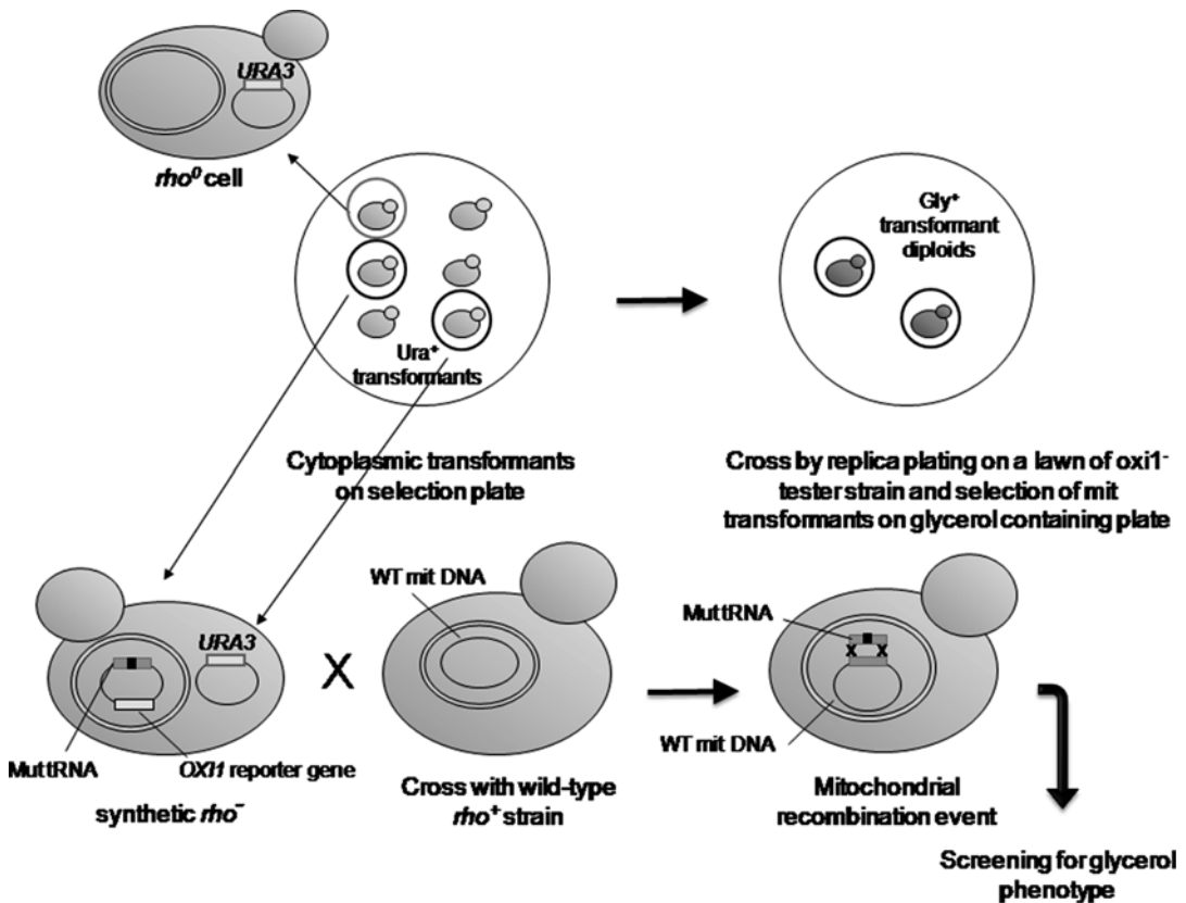
Fig 10.3 Schematic diagram for double selection of the transformants. In the first plate (ura - selective plate) are visualized colonies that have received the plasmid for nuclear selection. The transformants are crossed by replica plate with the tester oxi1 - strain (TF145). Only the diploids
