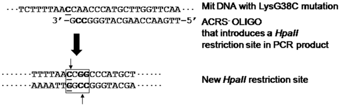
Fig 10.5 Example of ACRS strategy used for the selection of the tRNA Lys mitochondrial transformants. The new HpaII site ( boxed ) is introduced by PCR primer with
