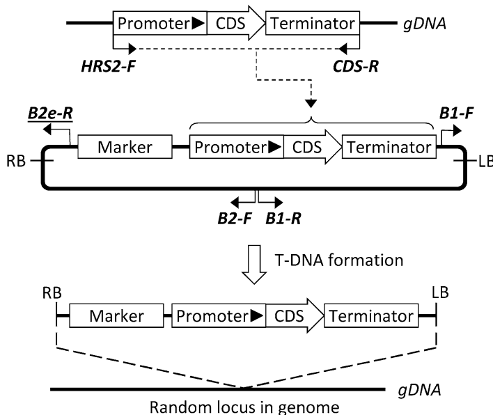
Fig. 14.1 Ectopic expression of a gene with its native regulatory elements. Primers are represented by solid arrows. CDS coding sequence of gene to be expressed, Term terminator region of gene to be expressed, gDNA genomic DNA, RB and LB right and left border repeats,
