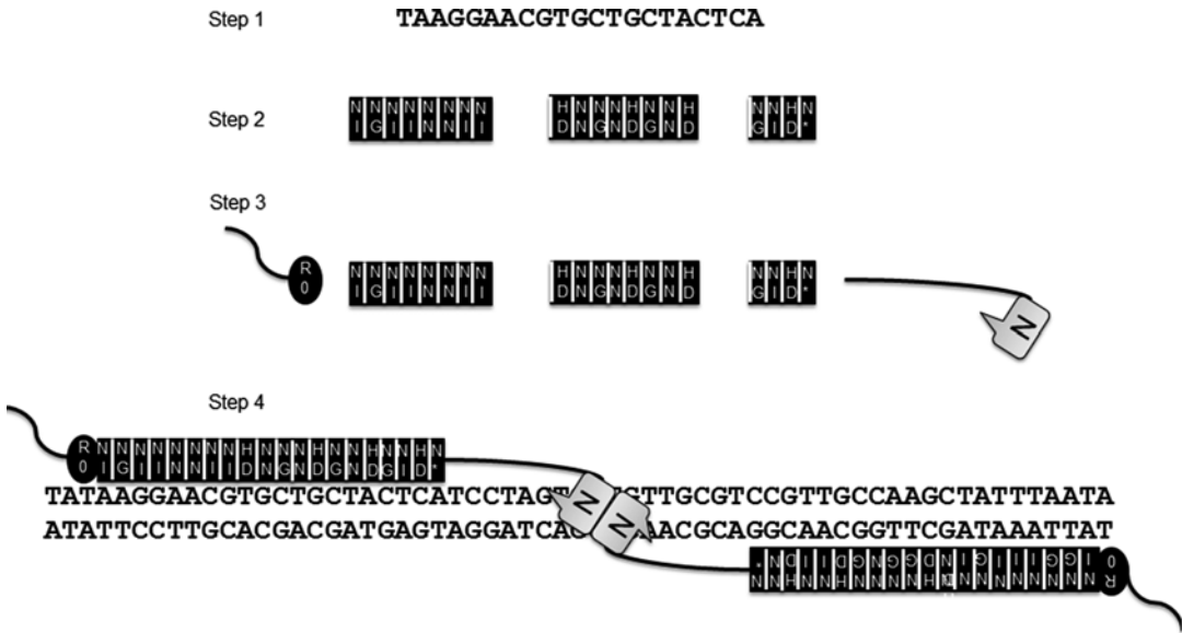
Fig. 27.5 TALEN assembly is depicted. Step 1, choose a target. Target half sites should begin with a T and contain a good mix of bases avoiding stretches of a single base or overly GC or AT rich sequence. The spacer between target half sites should be 18–20 bp. Step 2, using the Golden-Gate cloning method combine plasmids encoding RVDs for the target in sets of eight or less using the target sequence as a guide moving 5′–3′. Remember that R0 recognizes the first T and that R0 is encoded by the TALEN
