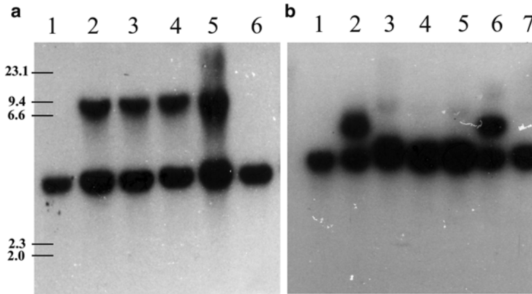
Fig. 6.2 Southern blot analysis of genomic DNA of N. crassa transformants digested with (a) Hind III and (b) Eco RI and hybridized with ^{32} P-labeled 2.4-kb
