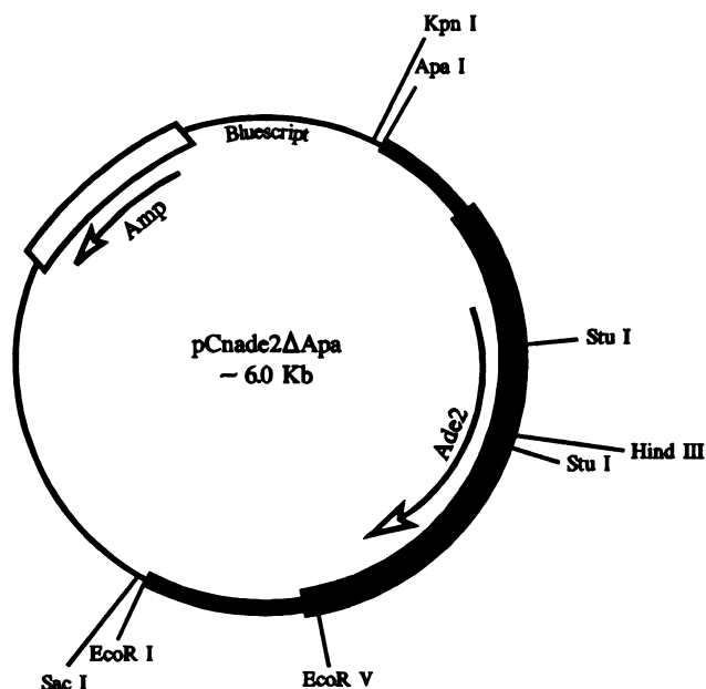
FIG. 1. Circular restriction map of the transforming plasmid pCnade2ΔApa, which contains an ≈3.0-kb insert of genomic ade2 from B-3501 cloned between the Apa I and Eco RI sites of Bluescript. The thick lines represent the genomic DNA insert, which contains the cryptococcal ade2 gene and flanking DNA. The thin line represents the Bluescript plasmid DNA.
