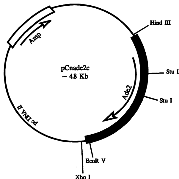
FIG. 2. Circular restriction map of the transforming plasmid pCnade2c, which contains an 1,822-bp cDNA insert from H99 ligated to Bst XI nonpalindromic linkers and cloned between the Bst XI sites of pcDNA II. The Bst XI sites are no longer present. The thick line represents the cryptococcal cDNA insert. The thin line represents the pcDNA II plasmid DNA.
