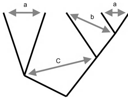
FIGURE 10.3 Independent contrasts. Contrasts are differences between sister taxa, as indicated by the gray arrow. For tips that share a common ancestor (a), they are the difference between sample means. For unpaired tips (b), they are the difference between that tip and the MRCA of its sister clade. For internal nodes (c), they are the difference between the respective MRCAs.
