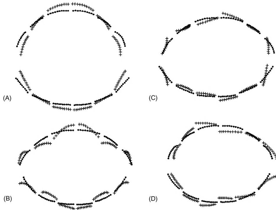
FIGURE 7.4 The first four SAs (A–D), showing patterns of covariation in the maxillary and mandibular dentition (occlusal view with maxilla at top).
