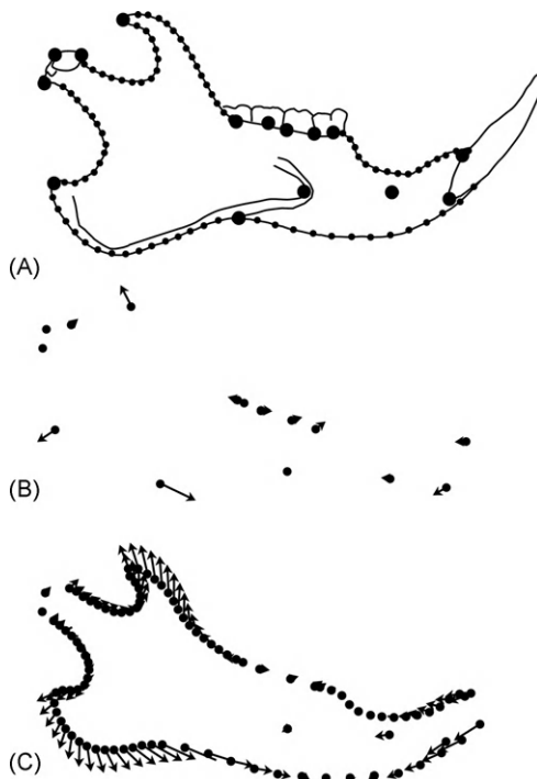
FIGURE 2.7 Ontogenetic shape change of the mandible of a ground squirrel, Spermophilus beecheyi . (A) Landmark and semilandmark measurement scheme (the larger dots are the landmarks); (B) ontogenetic change described by landmarks alone; (C) ontogenetic change described by landmarks, supplemented by semilandmarks.
