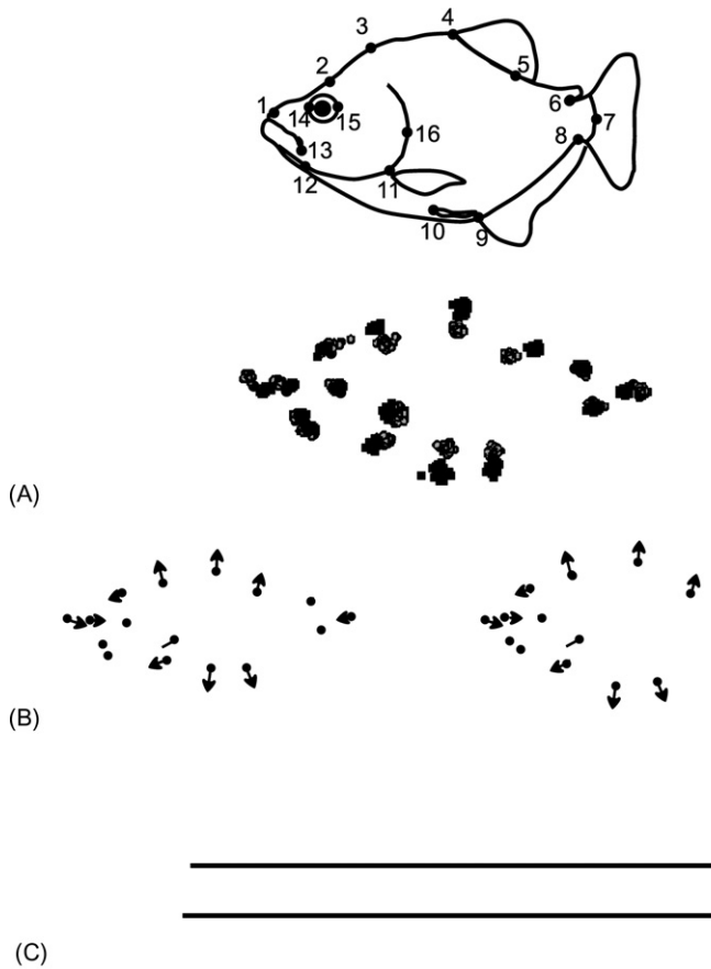
FIGURE 11.18 Change confined to early morphogenesis. (A) Superimposed coordinates of juvenile shapes; (B) ontogenies of shape; (C) lengths of ontogenetic vectors of shape. The two species differ in shape at the outset of the measured phase, but subsequently follow the same ontogeny of shape and do not differ in the length of their ontogenetic vectors.
