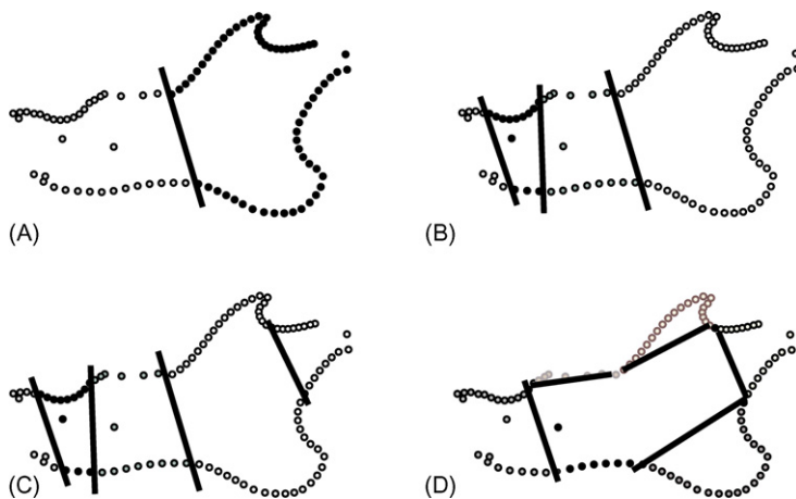
FIGURE 12.17 Four hypotheses of mandibular modularity. (A) Front/Back model; (B) Satb2 model; (C) Satb2 + Gsc model; (D) Condensation model. The black lines show the subdivisions between the modules.
