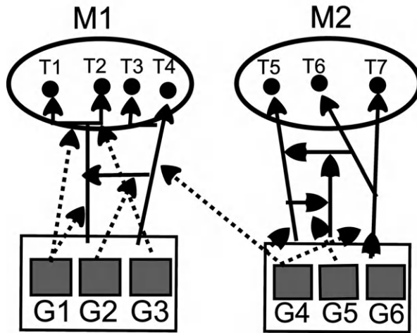
FIGURE 12.13 A developmental reframing of the classic concept of modularity, giving a developmentally explicit version of the genotype–phenotype map (after Klingenberg, 2008). There are two developmental modules (M1, M2) comprising two groups of traits (T1–T4, T5–T7). Genes affect developmental pathways rather than traits; the impact of the gene on a pathway is shown as a dotted line intersecting a pathway, shown as a solid line. A direct interaction between pathways is shown as an intersection between solid lines.
