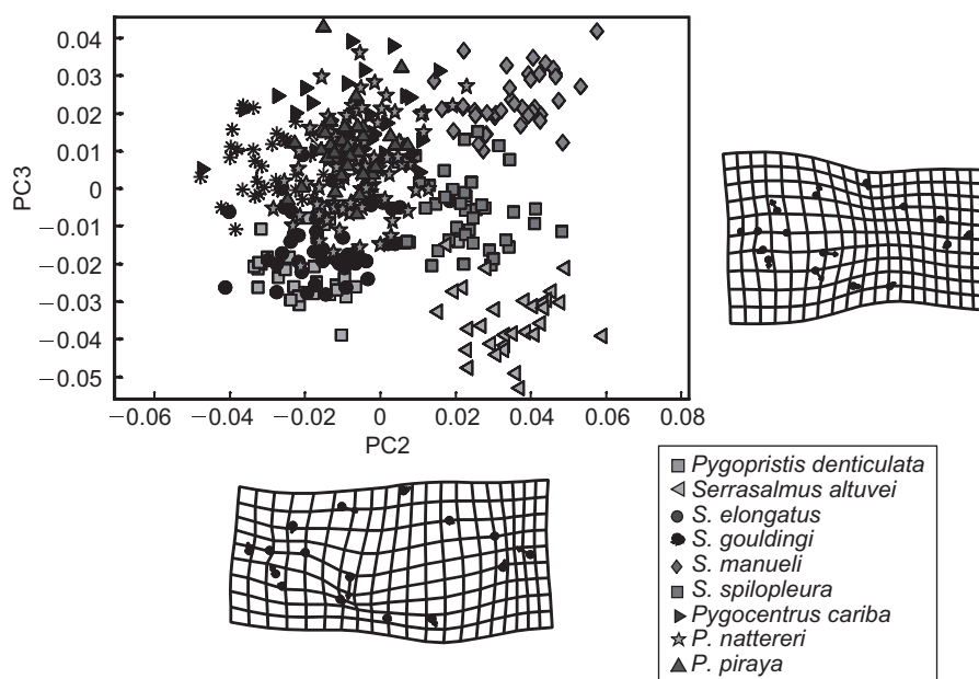
FIGURE 13.6 Scatter-plot of PC3 on PC2, and the deformations depicting these two dimensions of variation.
