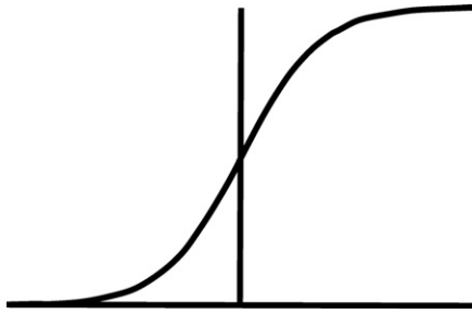
FIGURE 11.24 A sigmodal (logistic) growth curve.
