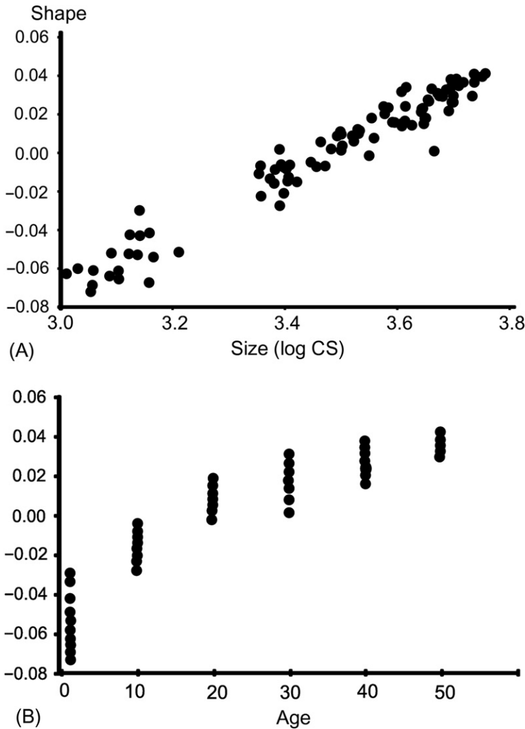
FIGURE 11.4 Projecting the three-dimensional trajectory onto a pair of planes, shape versus size, measured as log centroid size and shape versus age.
