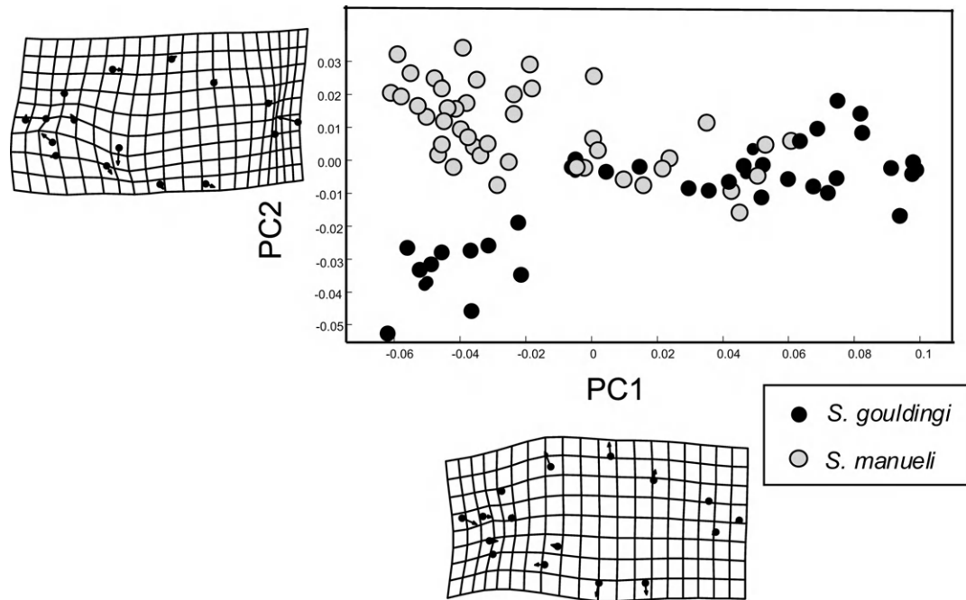
FIGURE 11.15 Principal components analysis of geometric shape data, pooling the ontogenetic series of S. gouldingi and S. manuei .
