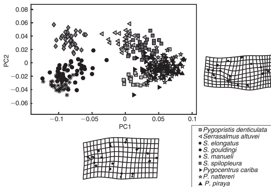
FIGURE 13.4 Principal components of body shape of nine species of piranhas; data were standardized and variation is examined among juvenile shapes (at the transition from larval to juvenile phases).
