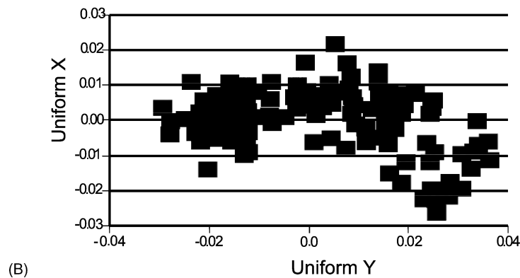
FIGURE 8.3 Checking the assumption of multivariate linearity of the dependent variable: (A) using principal components analysis; (B) using two shape variables on each other (the two uniform components).
