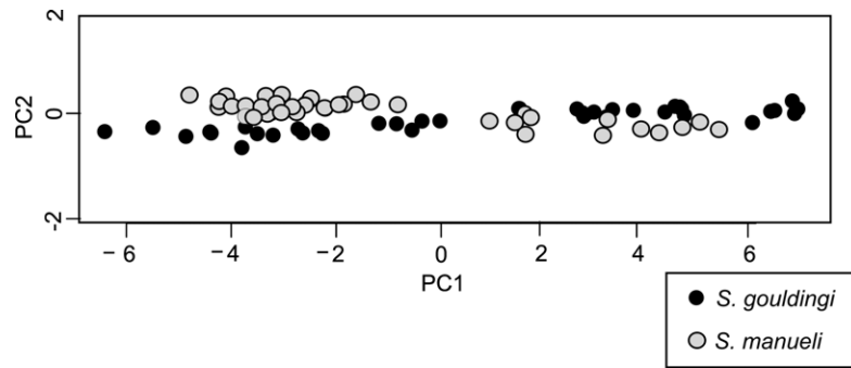
FIGURE 11.13 Principal components analysis of the traditional measurements, pooling the ontogenetic series of S. gouldingi and S. manuei .
