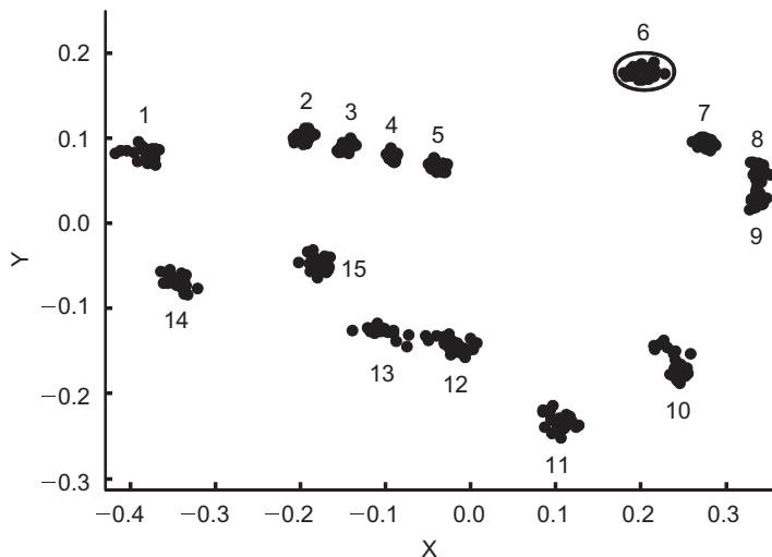
FIGURE 6.6 Plot of landmark coordinates of 31 S. niger jaws after partial Procrustes superimposition. The locations of landmark 6 in all 31 specimens are enclosed by an ellipse. Similar ellipses could be drawn for each landmark.
