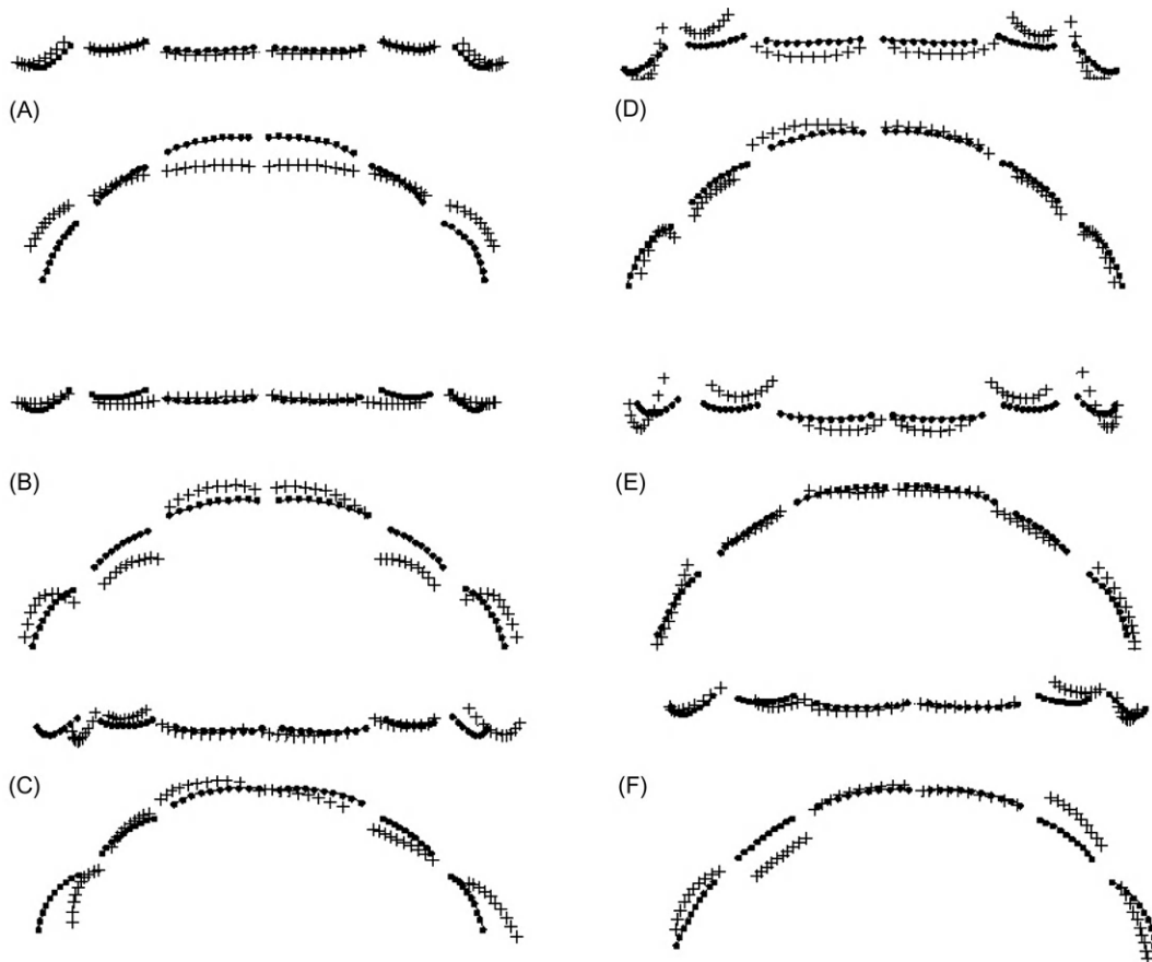
FIGURE 7.2 PCs 1–6 (A–F) of the maxillary dentition in frontal and occlusal views (see Figure 7.1 ). The data for the PC axis variation are shown as floating gray crosses. The average dentition over the entire set is shown as a series of black dots connected by solid lines along the incisal edges. The crosses indicate the pattern of differences for specimens with positive scores along the axis; specimens with negative scores would have the reversed pattern. It should be noted that the data shown in Figures 7.2 and 7.3 are three-dimensional in nature and that rotation in three-dimensional space permits a better understanding of the shape variance.
