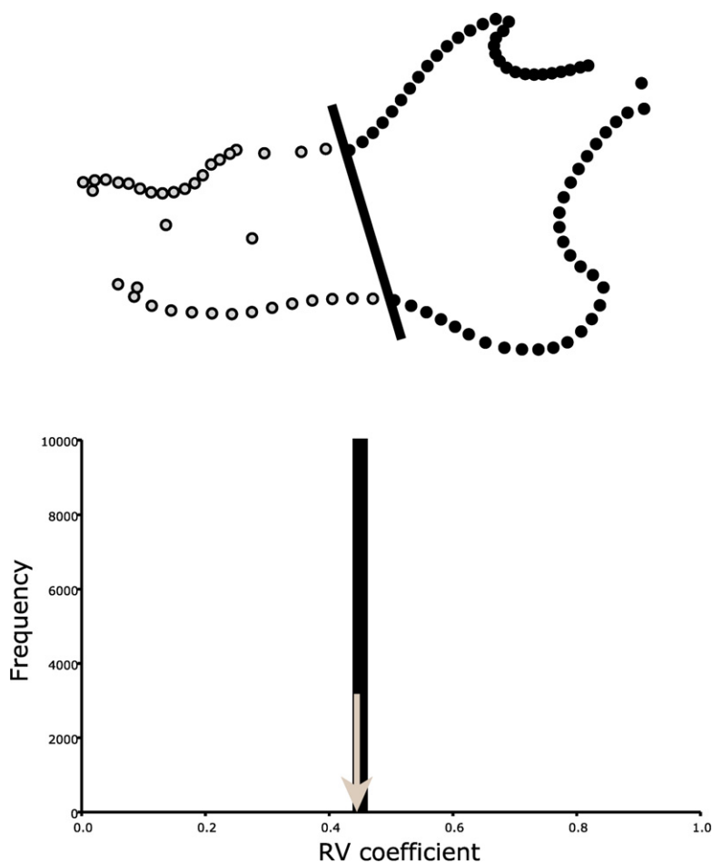
FIGURE 12.18 The distribution of the RV for the model and 10 000 randomly selected alternative subdivisions of the mandible into two parts having the same numbers of landmarks within each partition as contained in the model.
