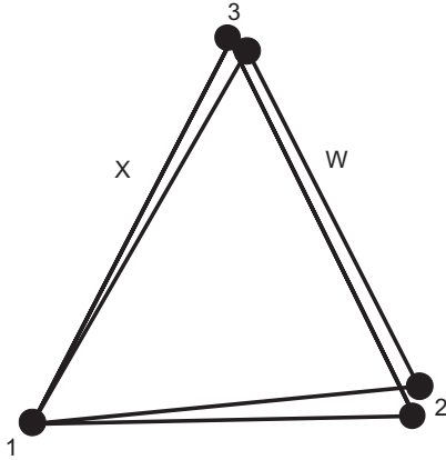
FIGURE 4.16 Triangles X and W after rotation of W to minimize the Procrustes distance. Computation of the landmark coordinates of W after rotation is given in Equation 4.24; the result is given in Equation 4.26. Vertices are numbered to indicate their homology.
