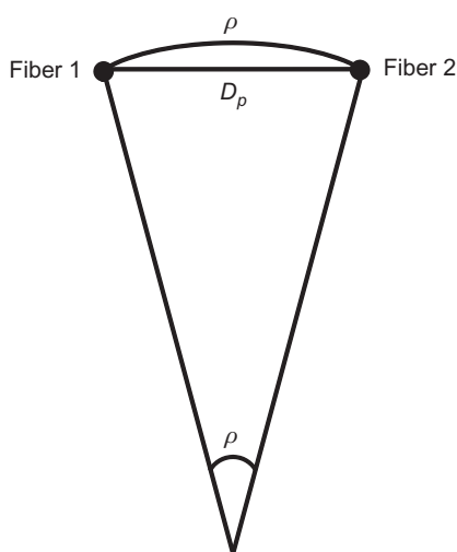
FIGURE 4.8 A slice through pre-shape space showing the Procrustes distance ( \rho ) and the partial Procrustes distance ( D_\rho ).
