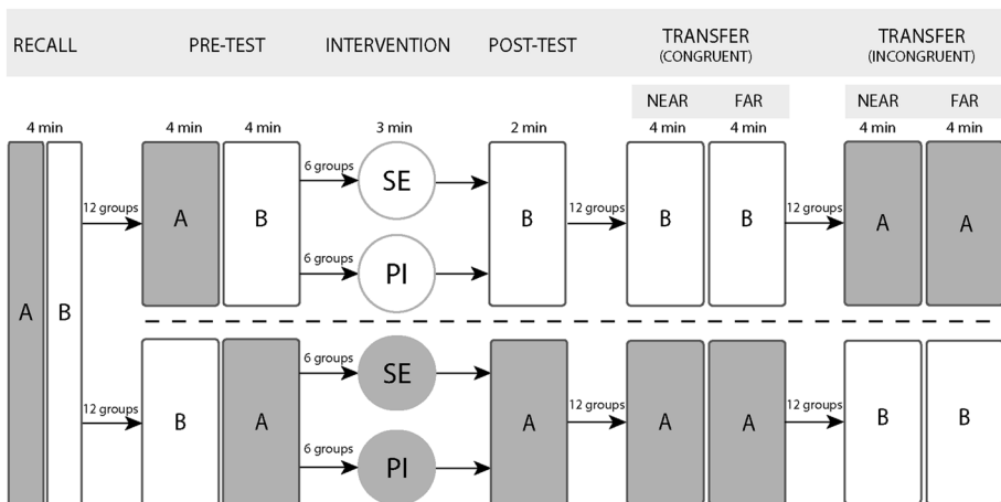
Fig. 1 Study design
