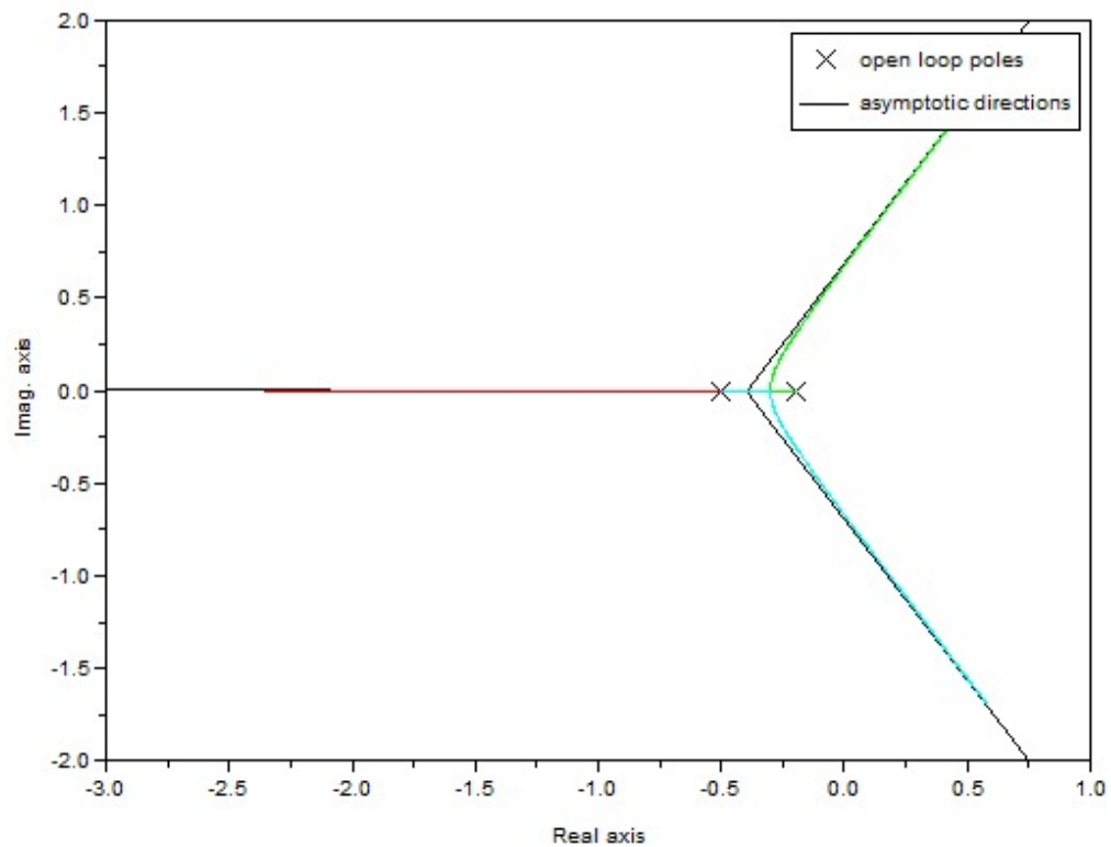
Evans root locus
