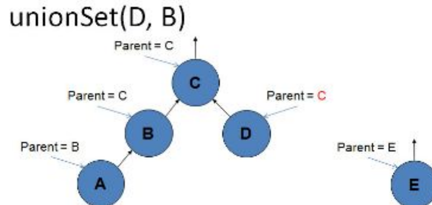
Figure 2.4: Calling unionSet(i, j) to Union Disjoint Sets
