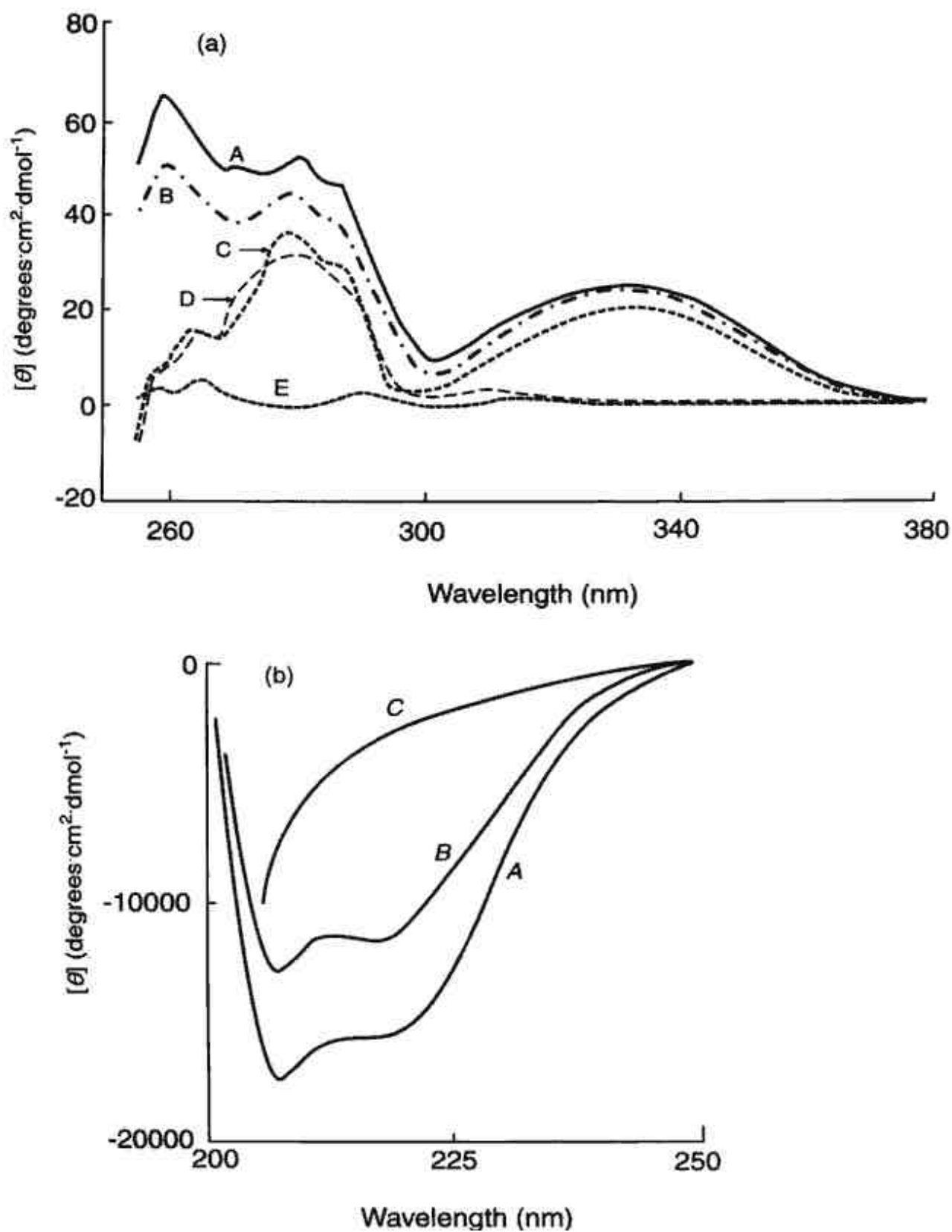
Fig. (5). The unfolding of phosphorylase b by GdmCl monitored by CD. (a) CD spectra over the range 255 to 380 nm were recorded in the absence of GdmCl and in the presence of 0.1 M ( ), 0.1 M ( ••• ), 0.53 M (•••••), 0.8 M (– – –) and 3 M GdmCl ( ••••• ). (b) Far UV CD spectra recorded in the absence of GdmCl (A), and in the presence of 1 M (B) and 3 M (C) GdmCl.
