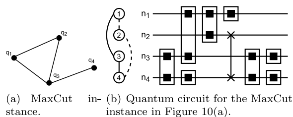
Fig. 10. Example of MaxCut instance (a) and one possible solution over the quantum hardware with 4 qubits (b left) represented by a quantum circuit (b right). Each binary gate must be executed on adjacent qubits, for this reason some swap gate (that represented by \times in the extremes) must be inserted.
