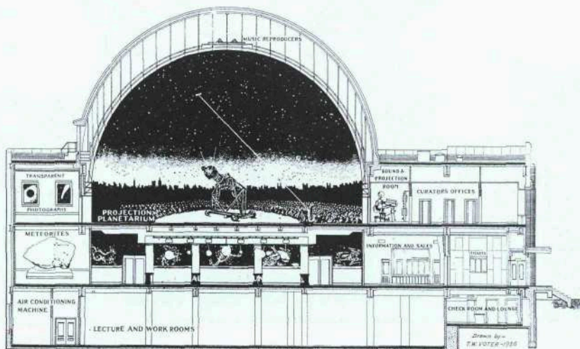
LONGITUDINAL SECTION OF THE HAYDEN PLANETARIUM
