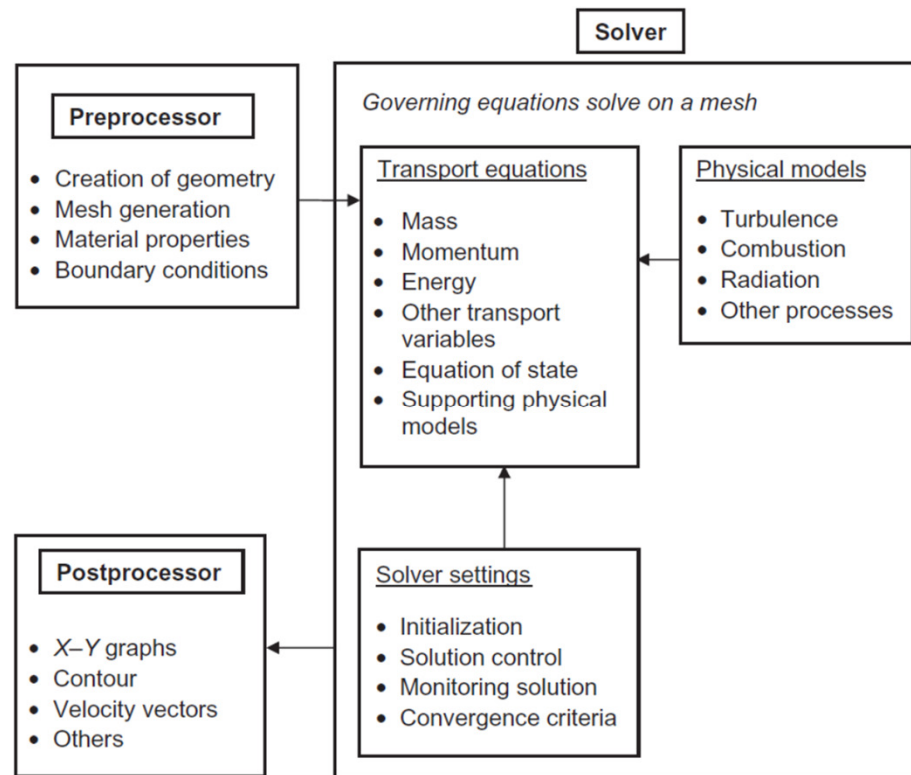
FIG. 2.1 The interconnectivity functions of the three main elements within a CFD analysis framework.
