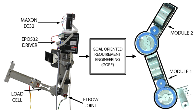
Fig. 2. The underlying idea of applying Goal Oriented Requirement Engineering (GORE), a software design tool borrowed from software engineering, for the integrated hardware and software design of a modular exoskeleton.
