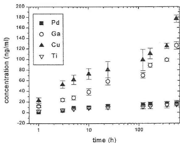
Figure 10 Ion release to the saliva from the palladium alloy.
