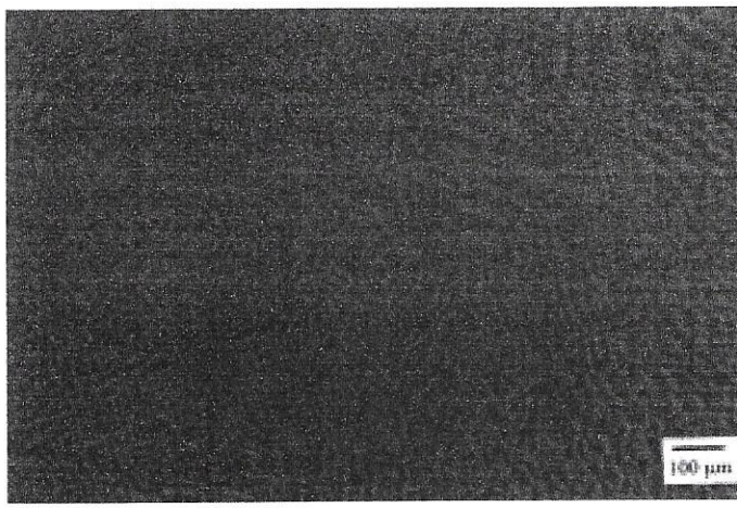
Figure 12 Microstructure of the nickel-chromium alloy.
