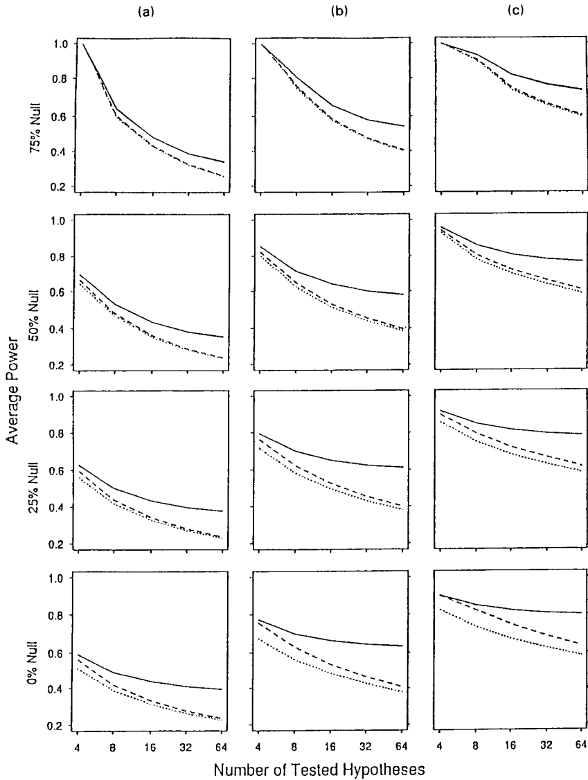
Fig. 1. Simulation-based estimates of the average power (the proportion of the false null hypotheses which are correctly rejected) for two FWER controlling methods, the Bonferroni (· · · · ·) and Hochberg's (1988) (----) methods, and the FDR controlling procedure (—): (a) decreasing; (b) equally spread; (c) increasing
