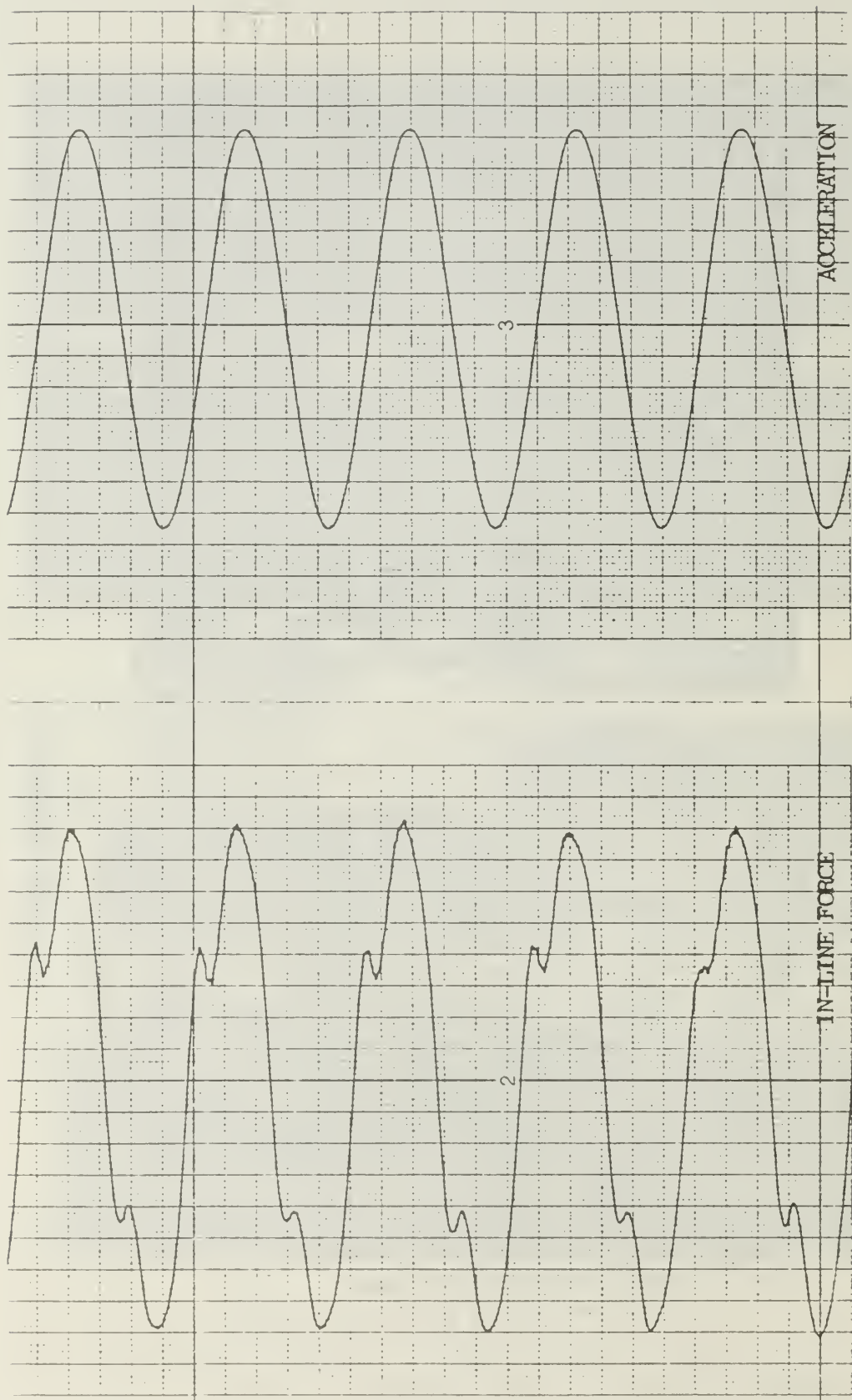
Fig. 8 Sample in-line force trace, K = 9.23 , k/D = 0 , \beta = 11,525 .
