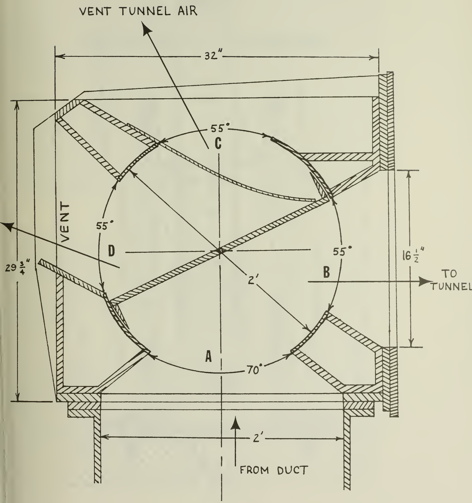
Fig. 4 Details of the three-way valve.
