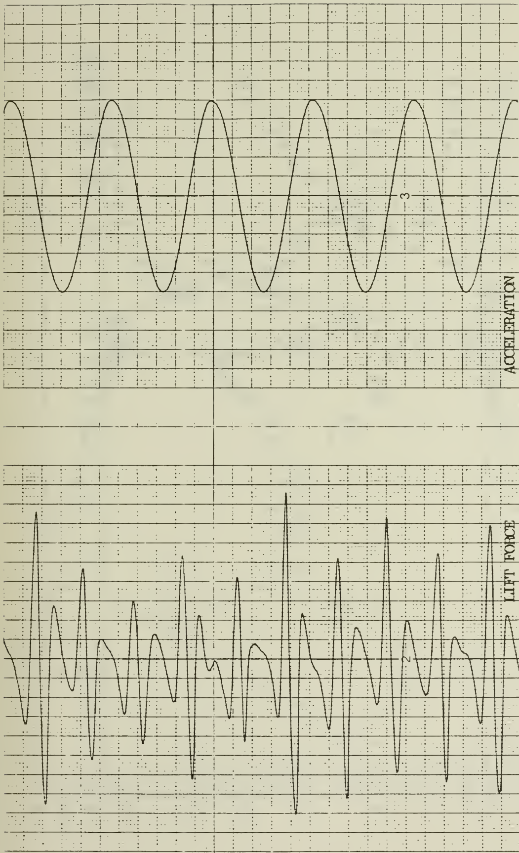
Fig. 15 Sample transverse force trace, K = 24.12 , k/D = 1/50 , \beta = 4924 .
