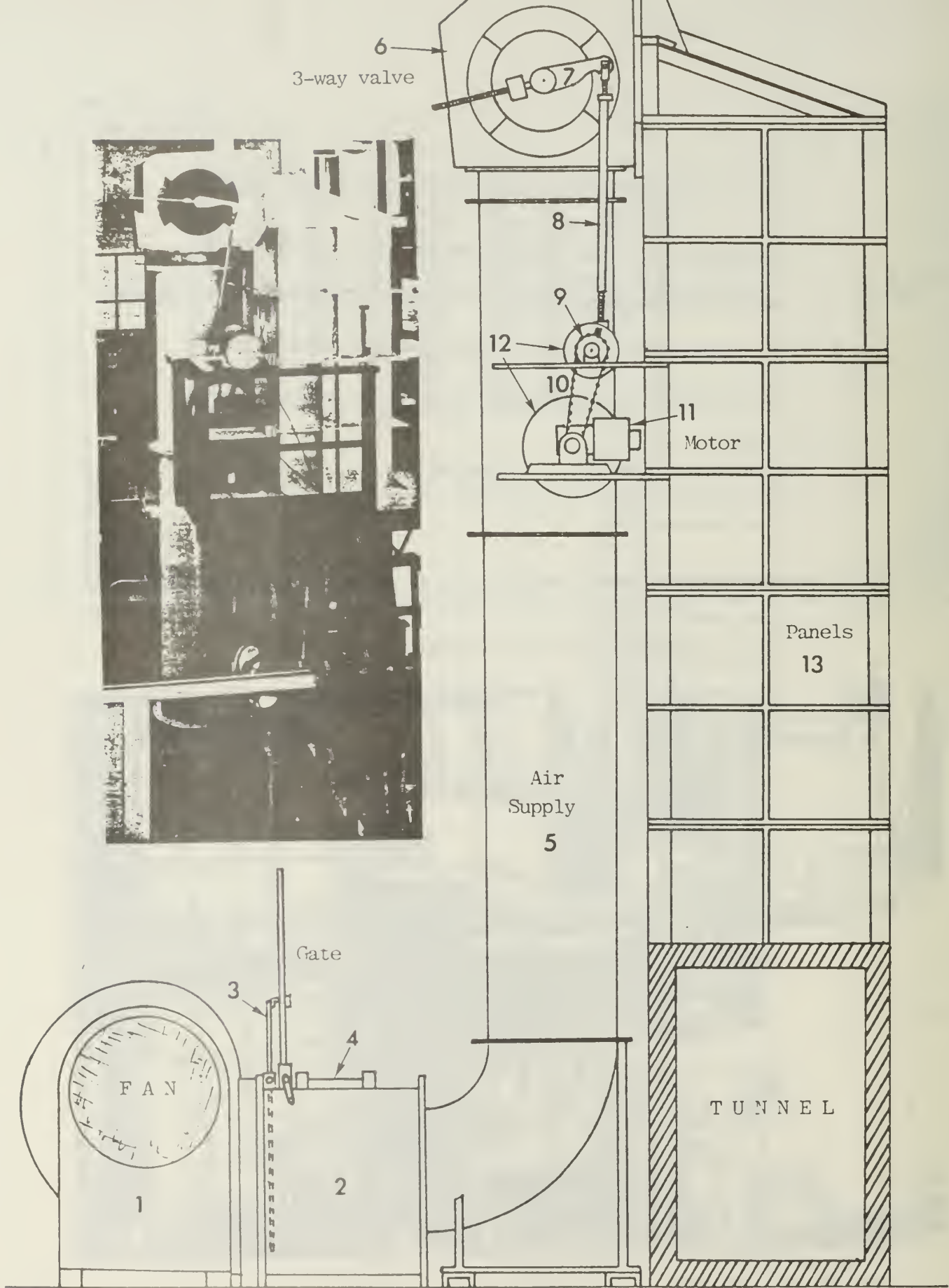
Fig. 3 Air supply system.
