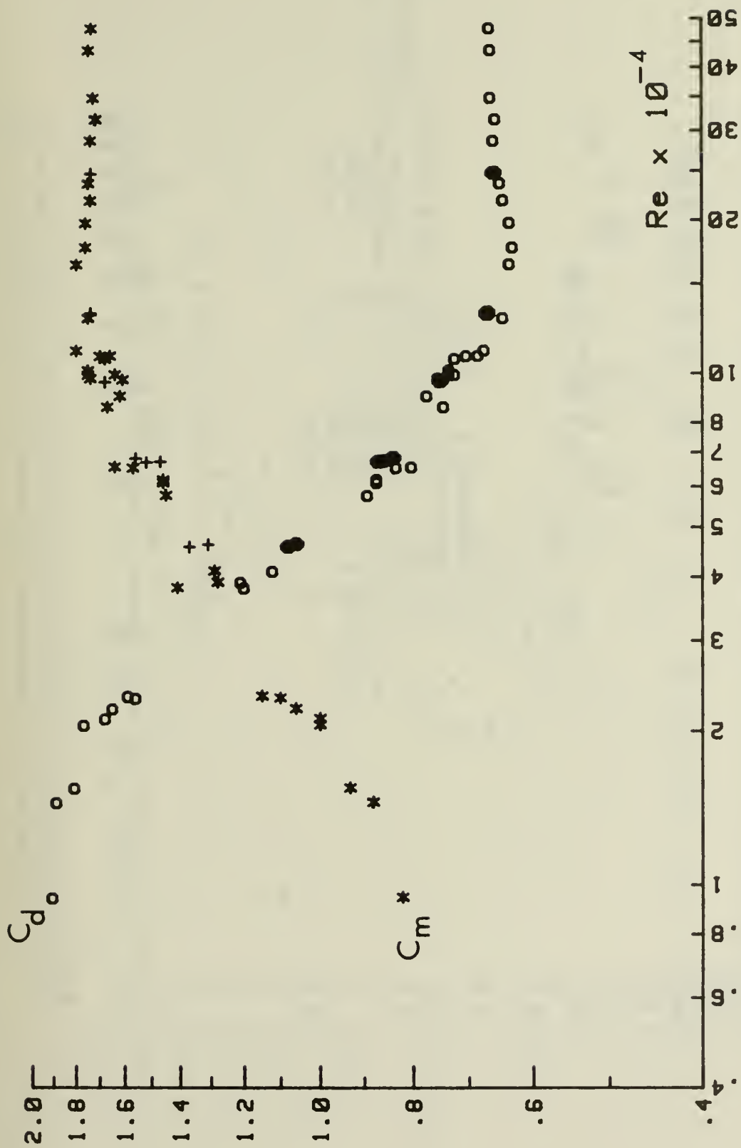
Fig. 23 Comparison of the present data with those reported in 1976 [1,2] for K = 20 , ● and +: Present data; ○ and *: 1976 data.
