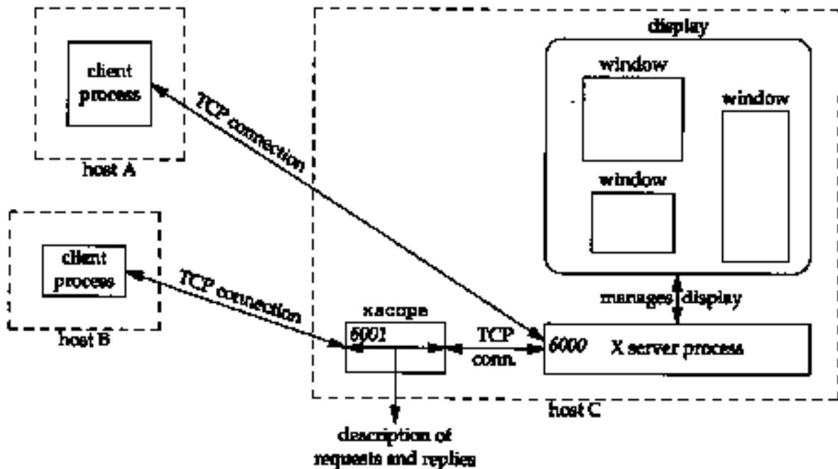
Figure 30.3 Using xscope to monitor an X connection.
