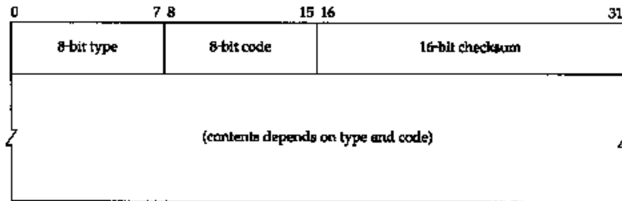
Figure 6.2 ICMP message.
