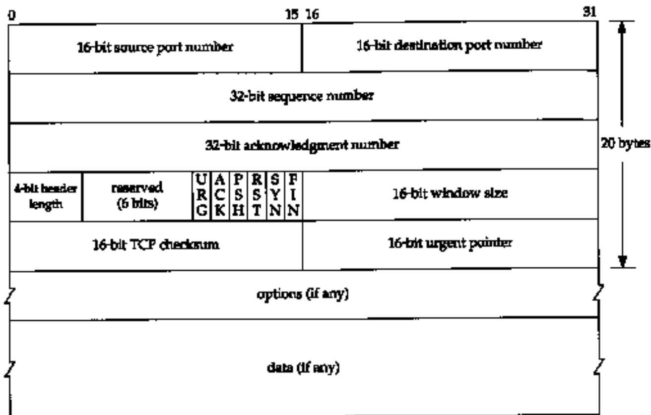
Figure 17.2 TCP header.
