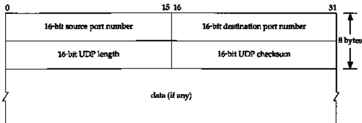
Figure 11.2 UDP header.
