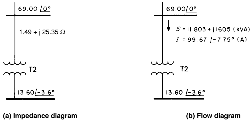
Figure 4-13—Impedance and flow diagrams
