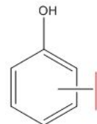
Fenol
