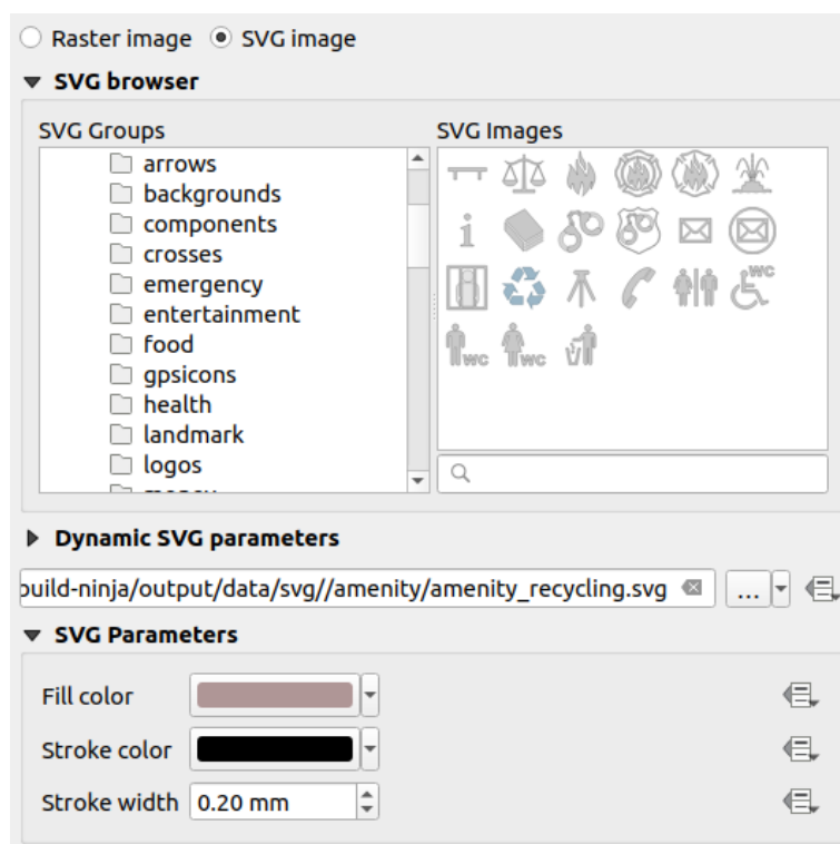
Figura19.50: Picture Item Properties panel
