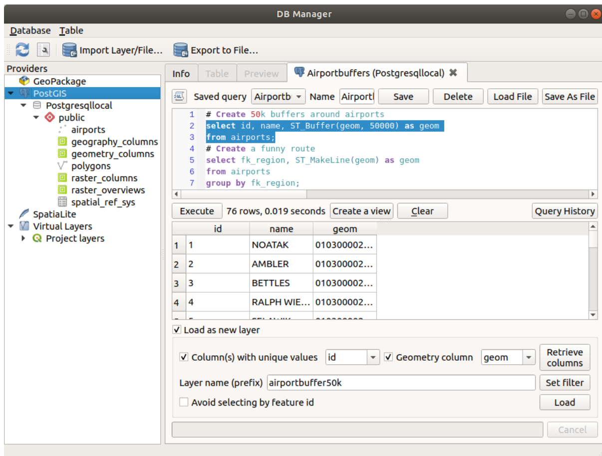
Figura26.9: Executing SQL queries in the DB Manager SQL window
