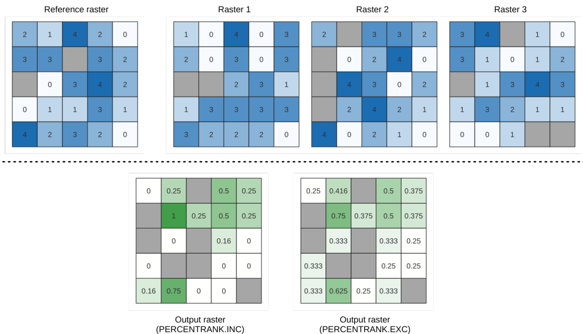
Figura25.10: Percent ranking Value = 1. NoData cells (grey) are ignored.
