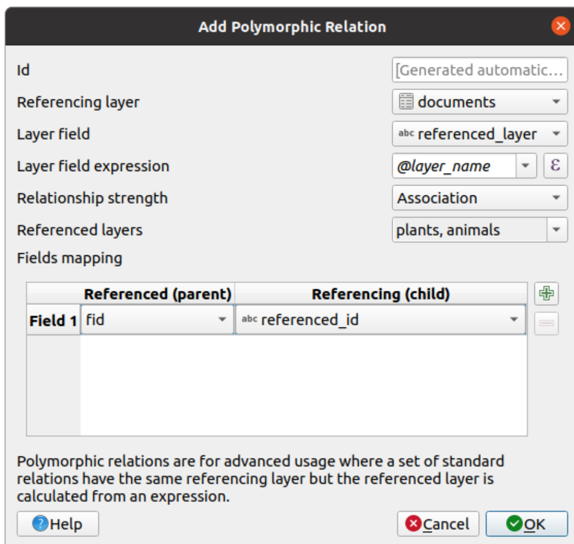
Figura15.83: Adding a polymorphic relation using documents layer as referencing and animals and plants as referenced layers.
