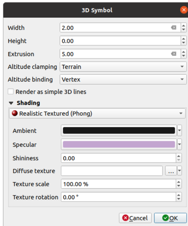
Figura13.30: Properties of a 3D line symbol
