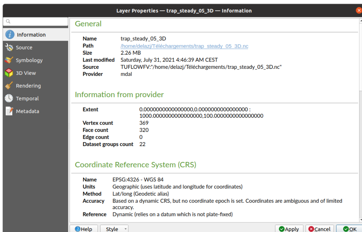
Figura 17.4: Mesh Layer Information Properties
