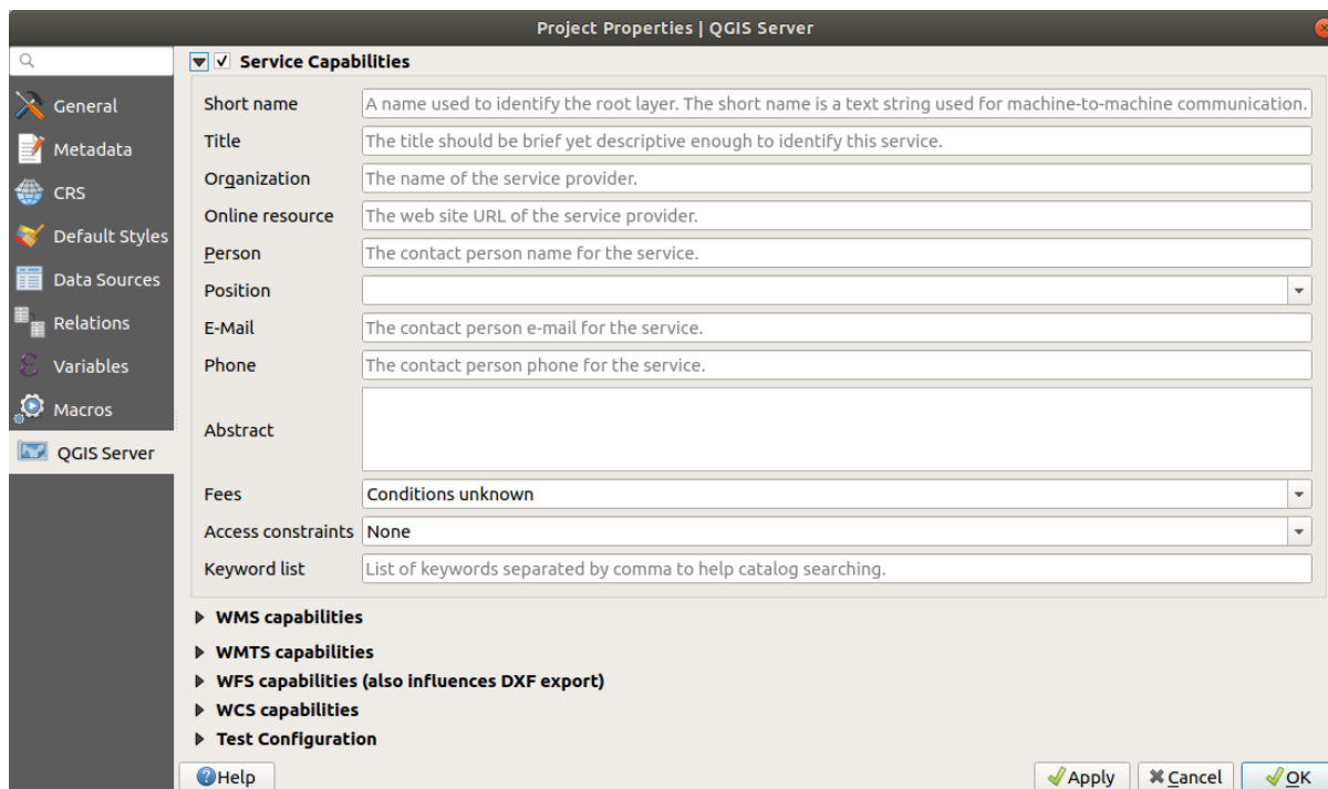
Figura9.31: QGIS Server settings tab
