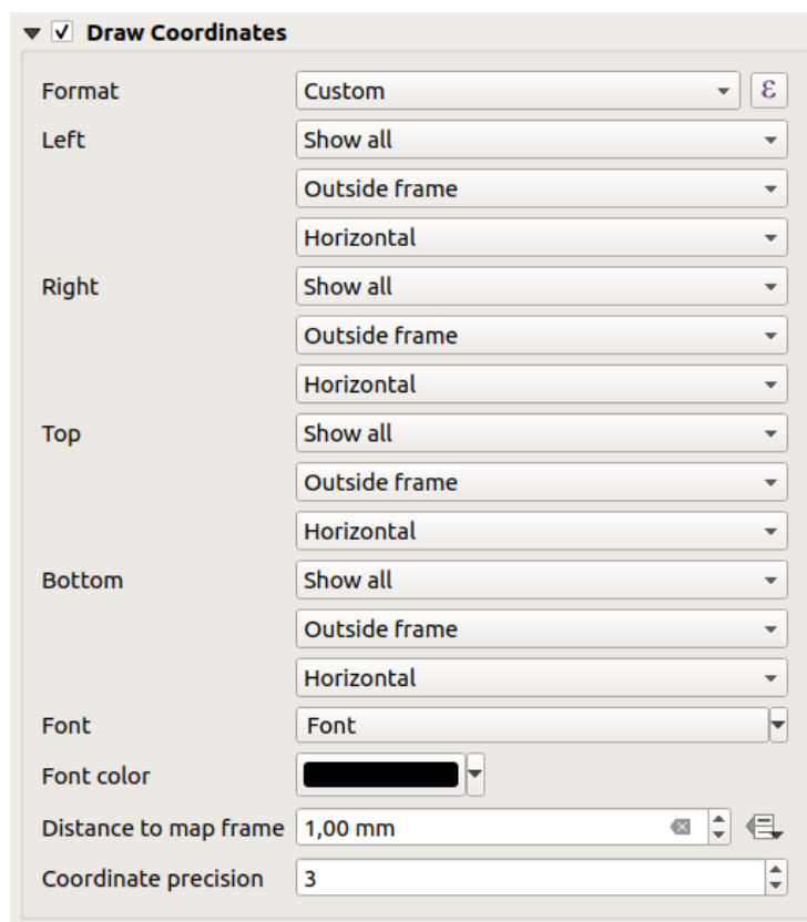
Figura19.21: Grid Draw Coordinates dialog
