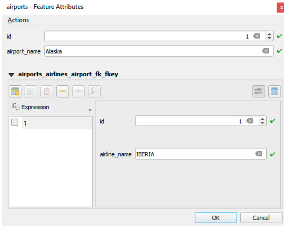
Figura15.82: N-M relationship between airports and airlines
