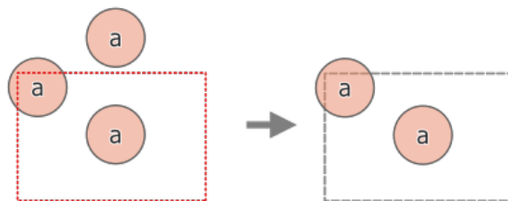
Figura25.103: Extract operation between a three-feature input layer “a” and a dashed extent (left) - resulting features with dashed extent for reference (right)
