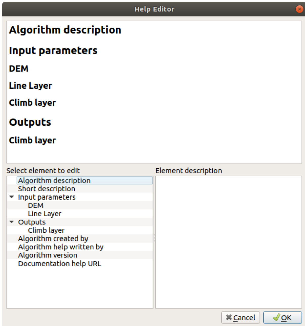
Figura24.25: Editing Help
