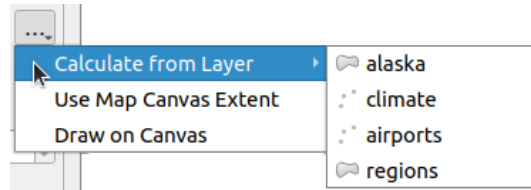
Figura24.11: Extent selector
