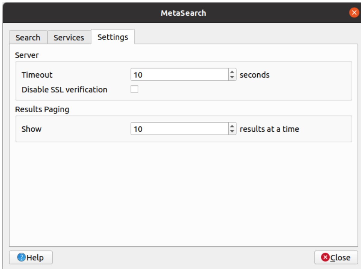
Figura26.16: MetaSearch settings
