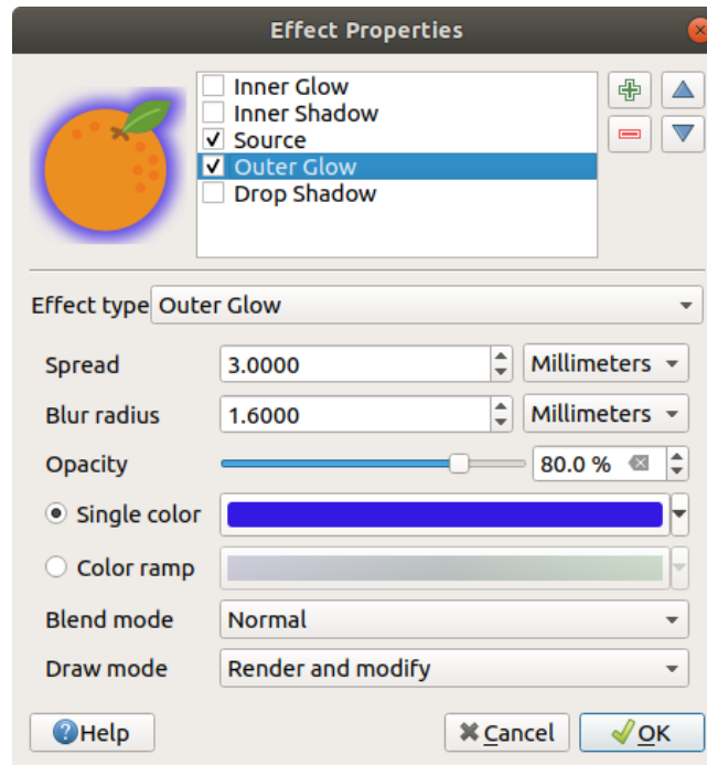
Figura15.23: Draw Effects: Outer Glow dialog
