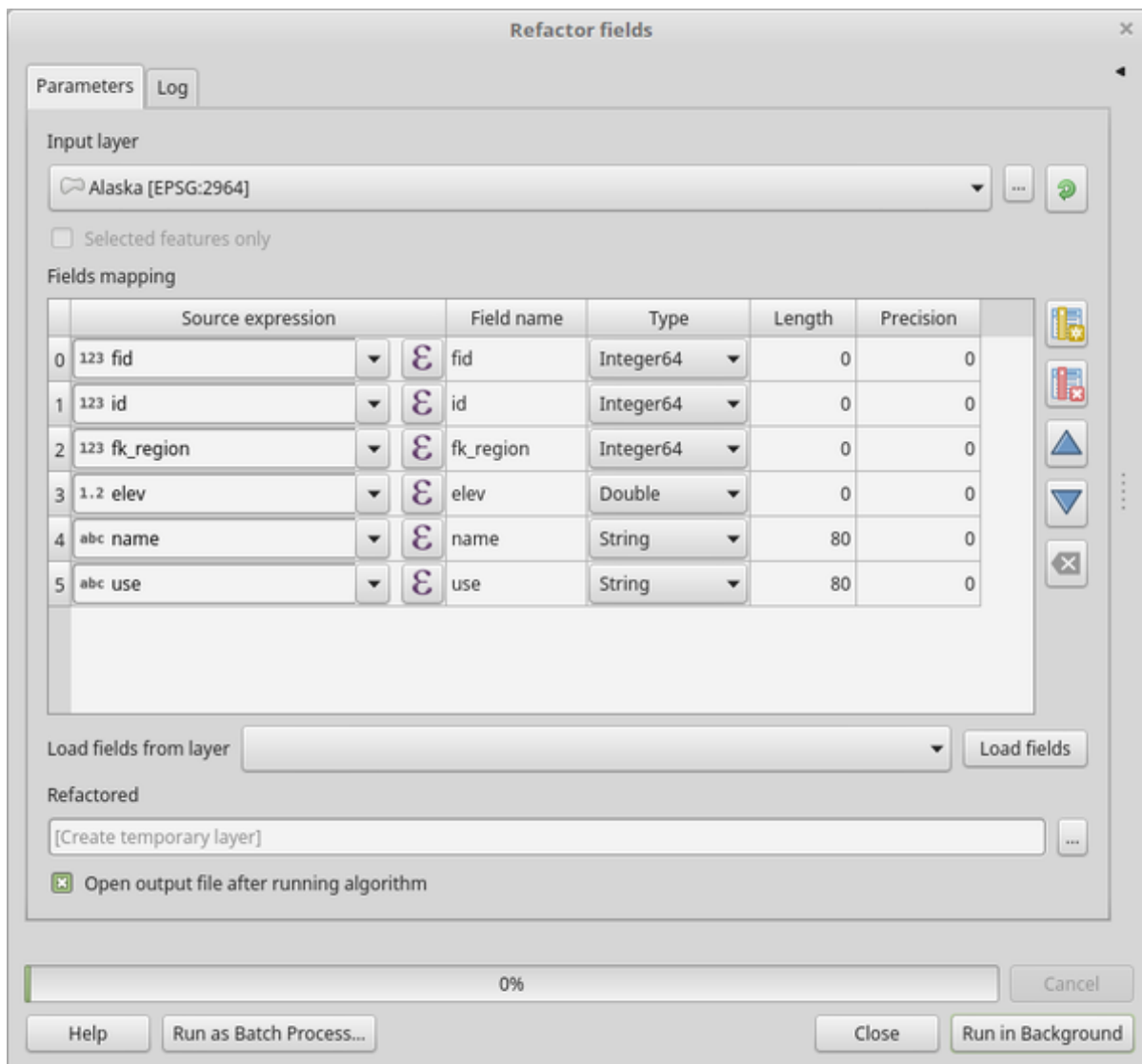
Figura25.113: Refactor fields dialog
