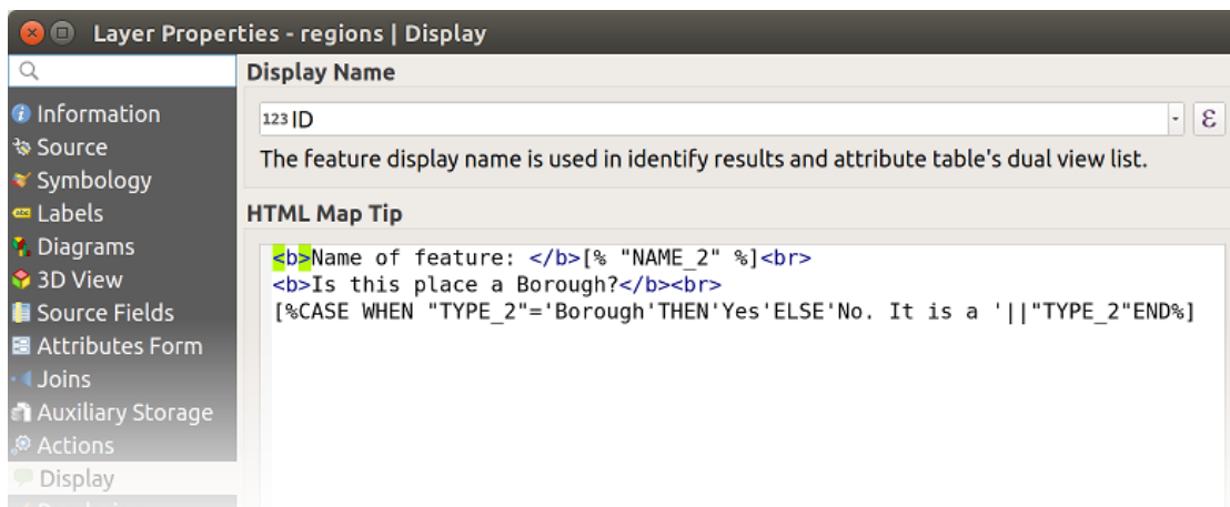
Figura15.58: HTML code for map tip
