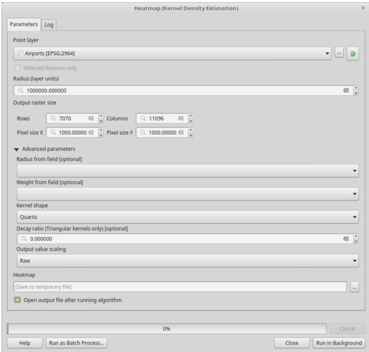
Figura25.3: The Heatmap Dialog
