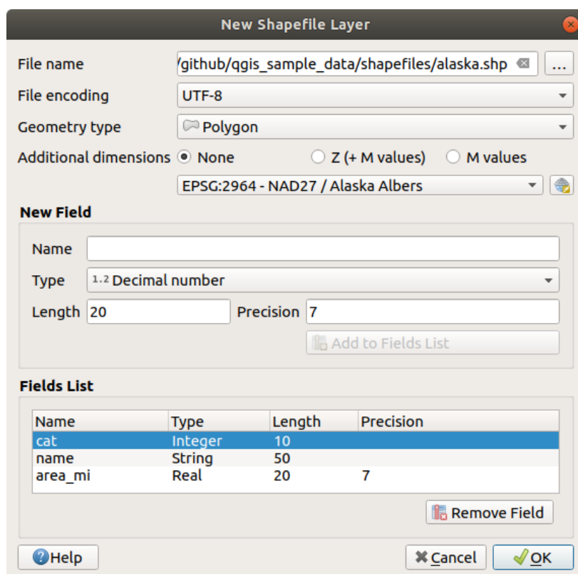
Figura14.18: Creating a new Shapefile layer dialog
