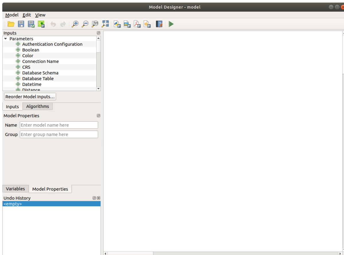
Figura24.16: Modeler
