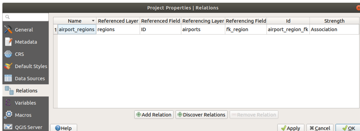
Figura9.29: Relations tab
