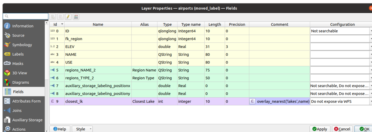
Figura15.40: Fields properties tab
