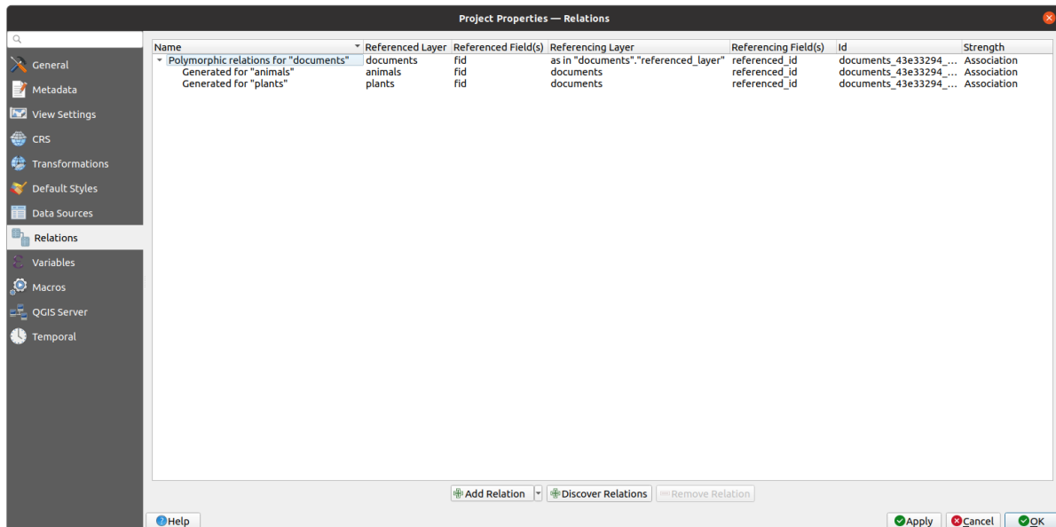
Figura15.84: Preview of the newly created polymorphic relation and its child relations for animals and plants.
