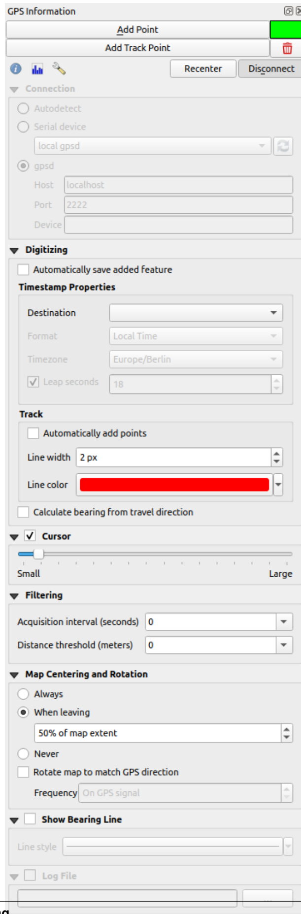
Figura21.5: GPS tracking options window
