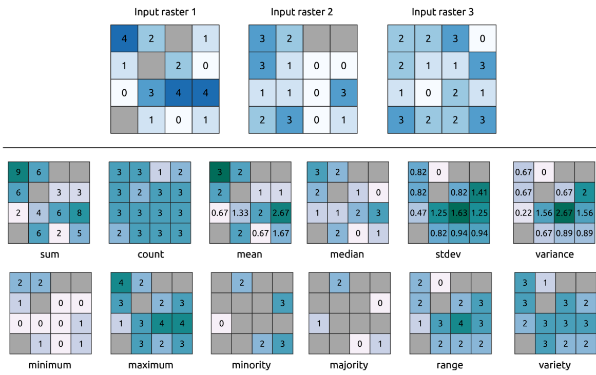
Figura25.13: Example with all the statistic functions. NoData cells (grey) are taken into account.
