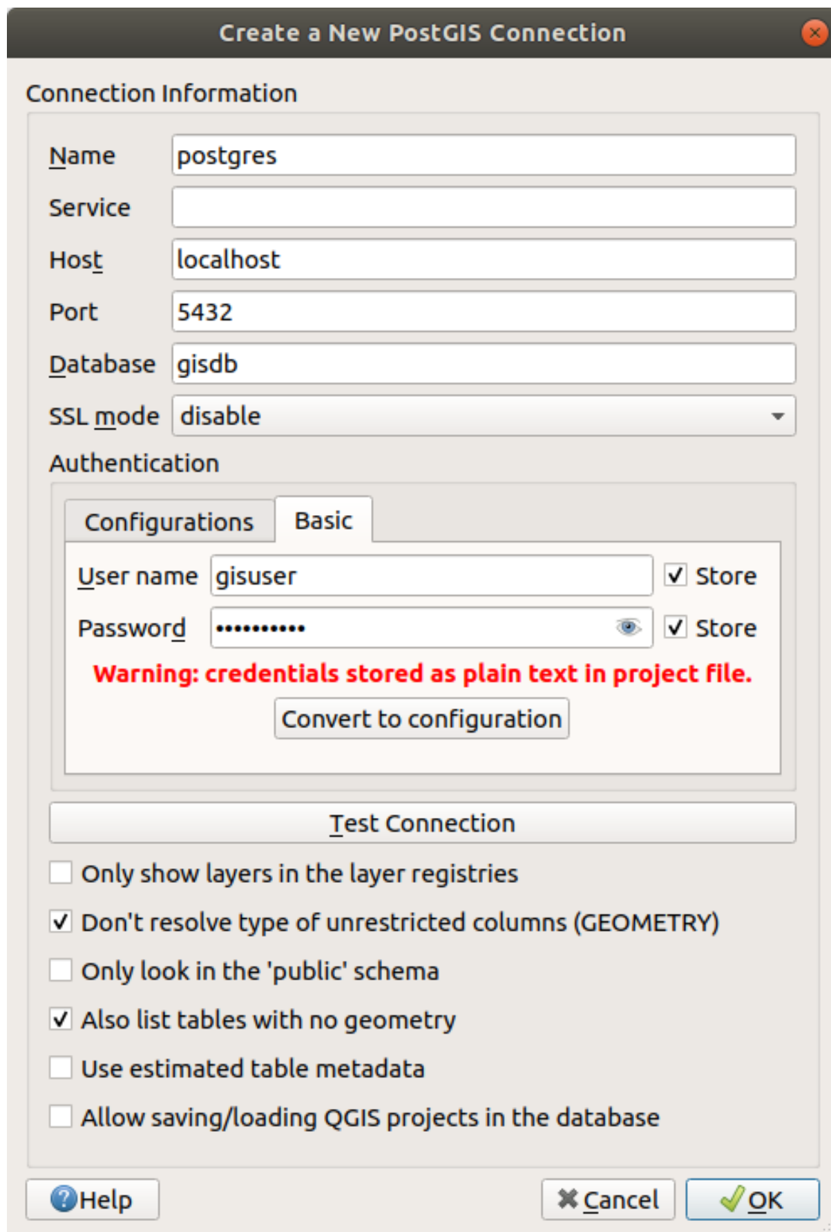
Figura14.12: Create a New PostGIS Connection Dialog
