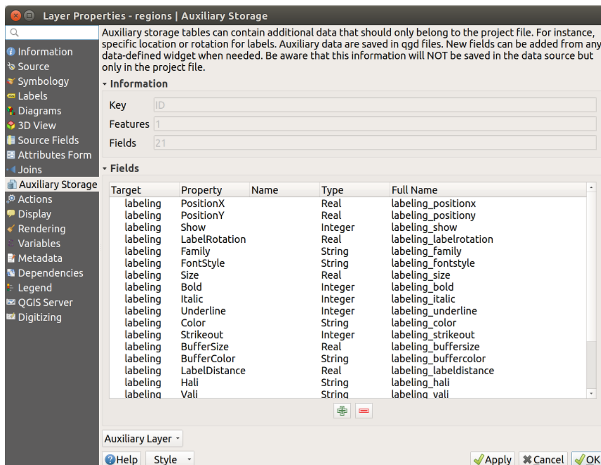
Figura15.48: Auxiliary Fields
