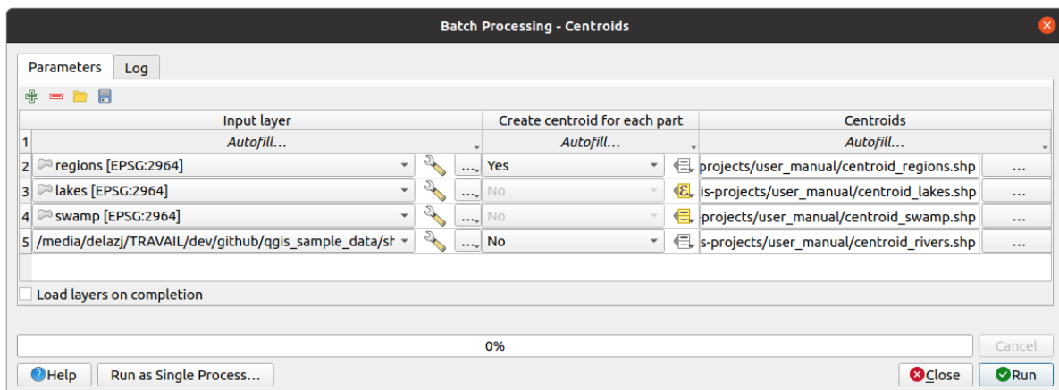
Figura24.31: Batch Processing
