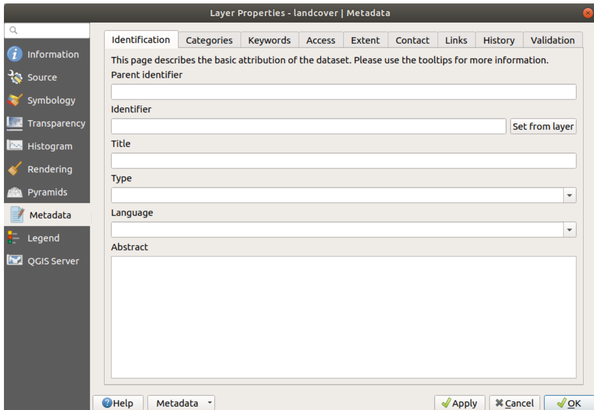
Figura16.17: Raster Metadata
