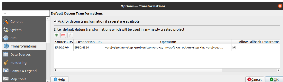
Figura9.4: Transformations Settings
