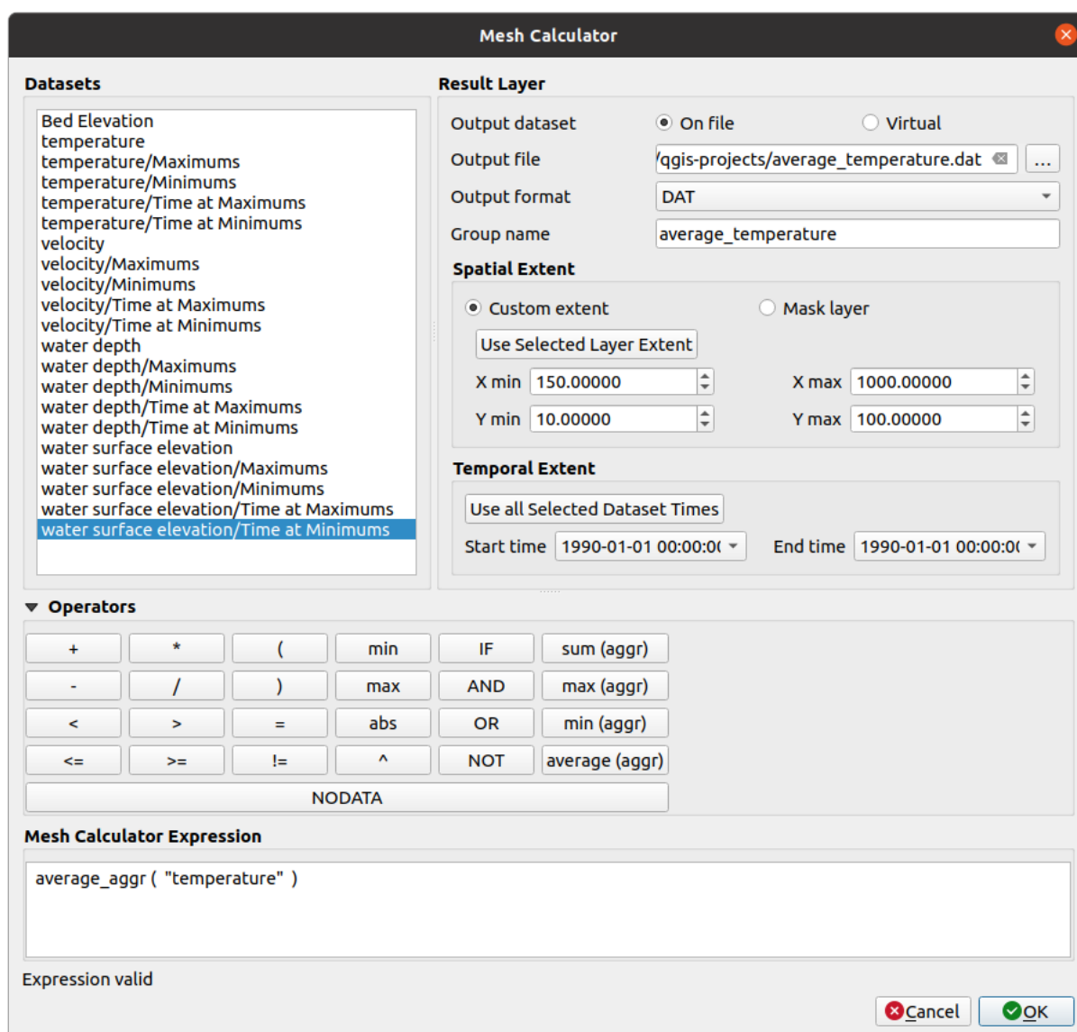
Figura17.12: Mesh Calculator
