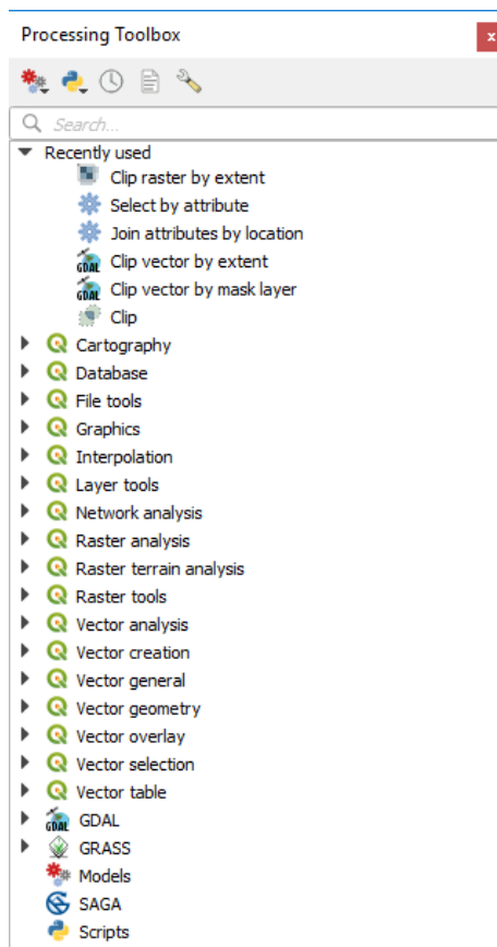
Figura24.6: Processing Toolbox
