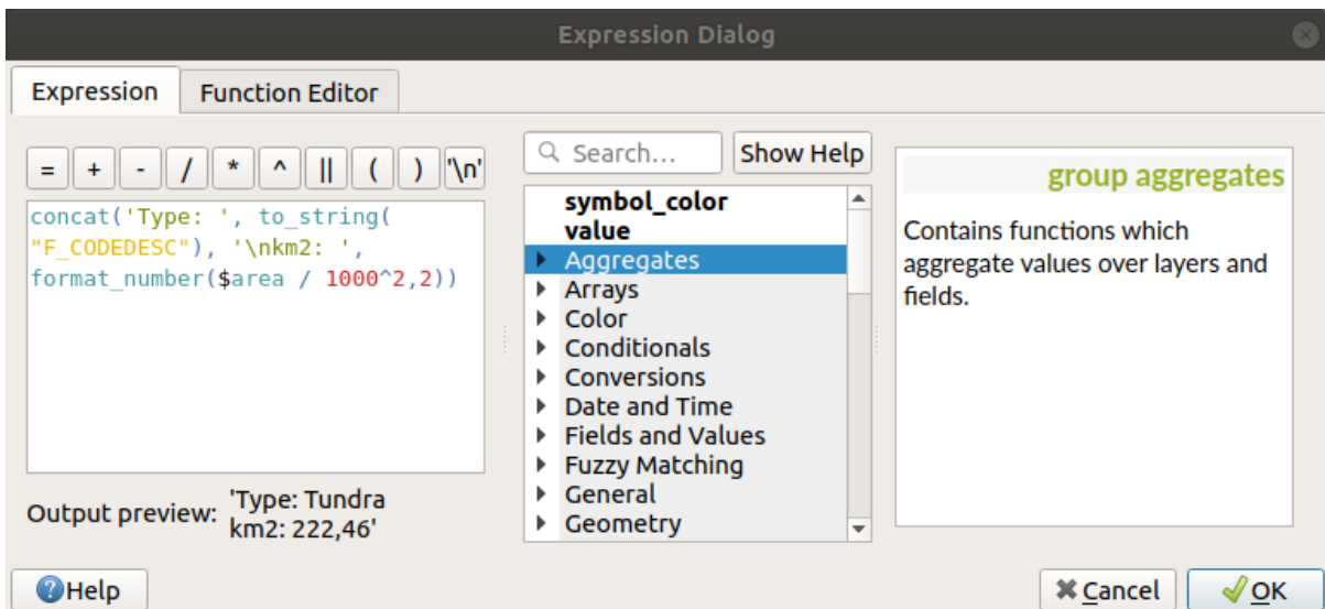
Figura15.29: Using expressions for labeling
