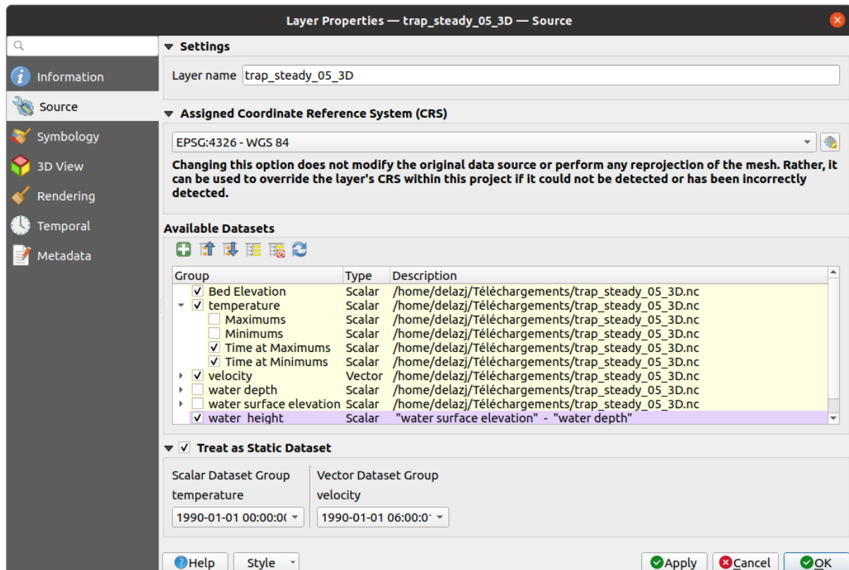
Figura17.5: Mesh Layer Source Properties
