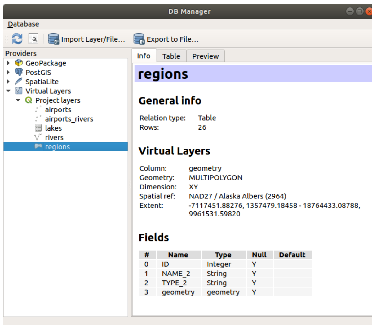
Figura26.8: DB Manager dialog
