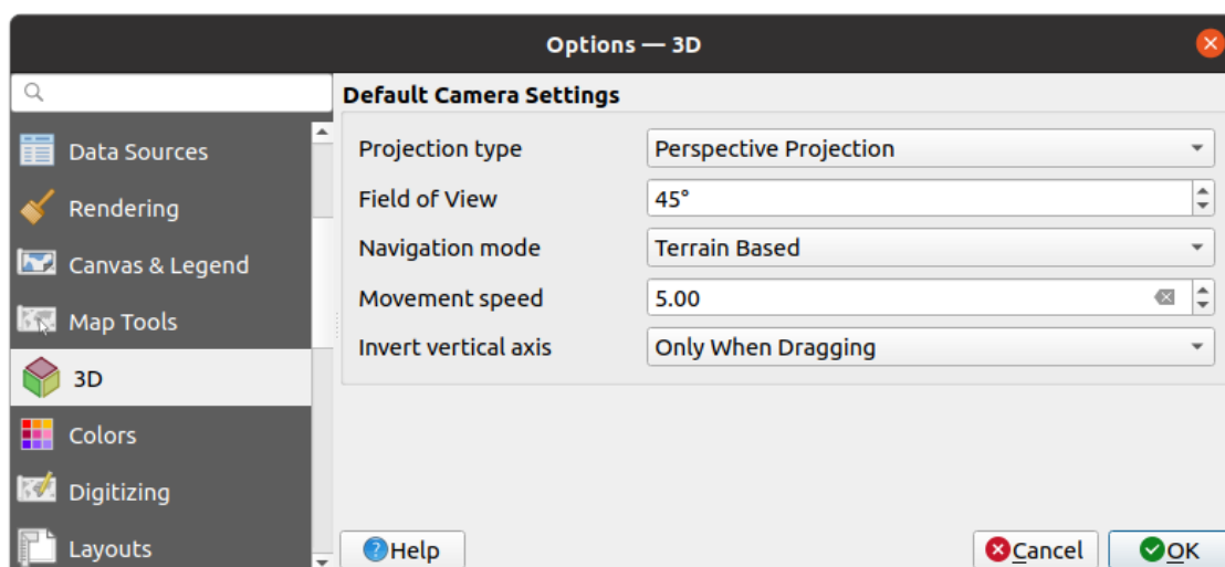
Figura9.9: 3D Settings
