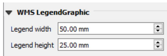
Figura19.32: WMS LegendGraphic
