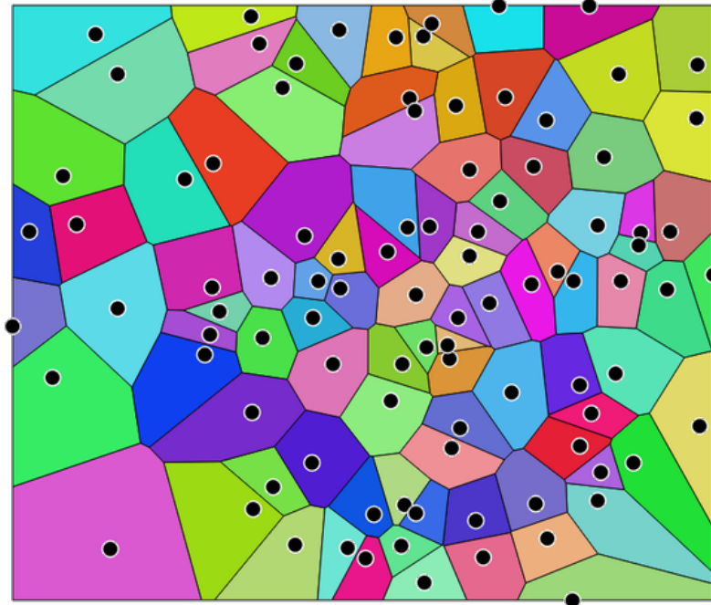
Figura25.100: Voronoi polygons
