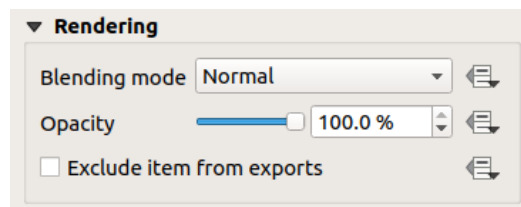
Figura19.13: Rendering mode
