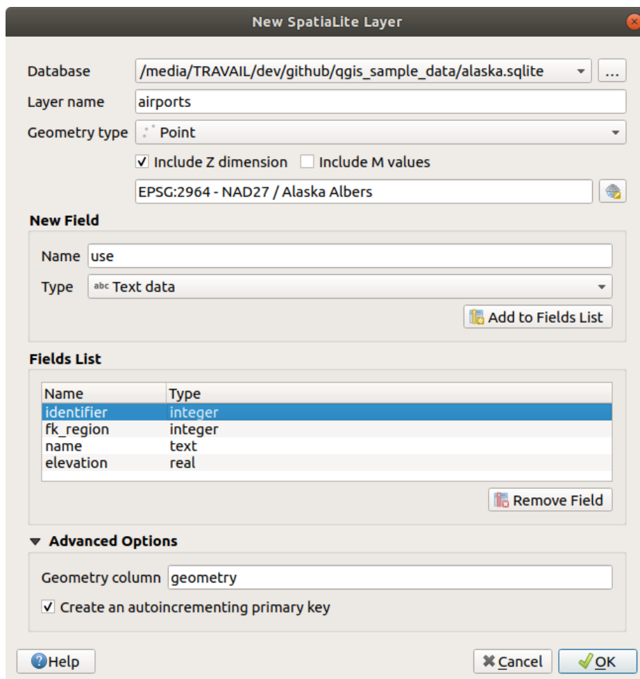
Figura14.19: Creating a New SpatiaLite layer dialog
