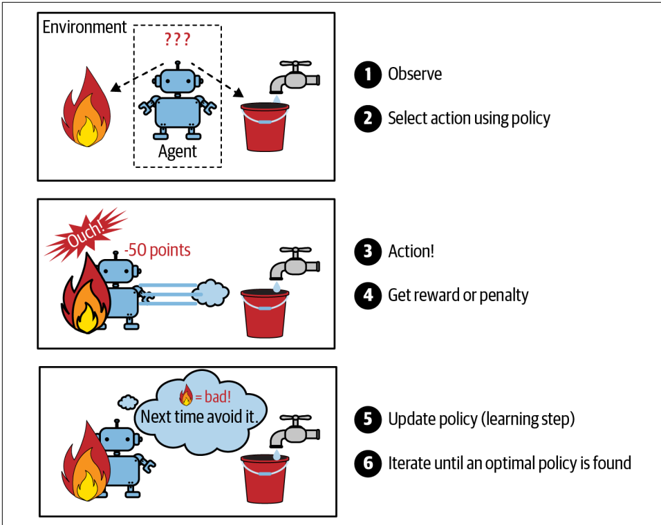
Figure 1-13. Reinforcement learning
