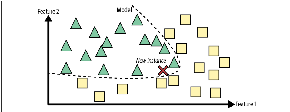
Figure 1-17. Model-based learning
