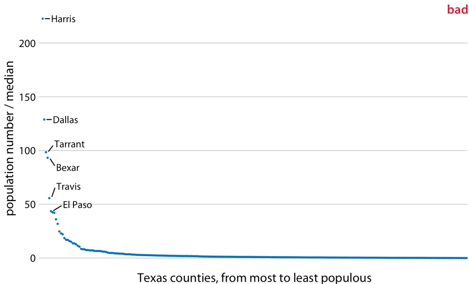
Figure 3-6. Population sizes of Texas counties relative to their median value. By displaying a ratio on a linear scale, we have overemphasized ratios > 1 and have obscured ratios < 1. As a general rule, ratios should not be displayed on a linear scale. Data source: 2010 US Decennial Census.
