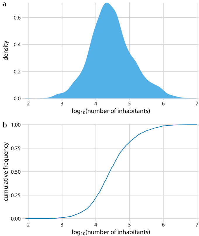
Figure 8-5. Distribution of the logarithm of the number of inhabitants in US counties. (a) Density plot. (b) Empirical cumulative distribution function. Data source: 2010 US Decennial Census.
