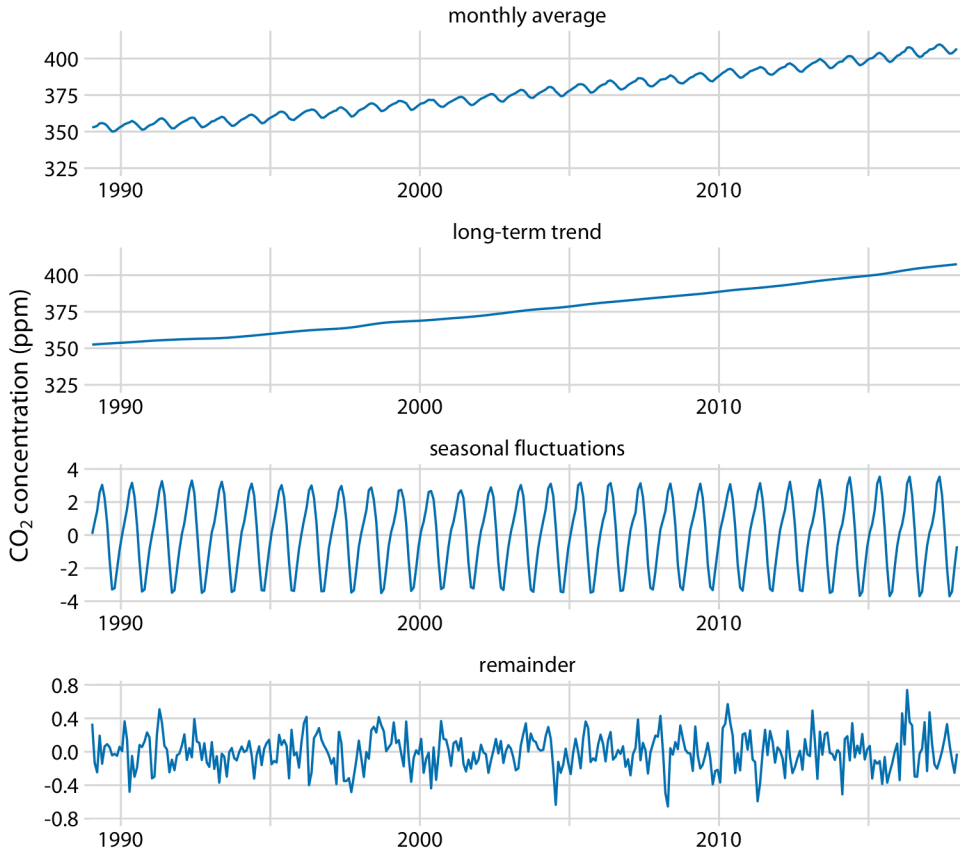
Figure 14-13. Time-series decomposition of the Keeling curve, showing the monthly average (as in Figure 14-12), the long-term trend, seasonal fluctuations, and the remainder. The remainder is the difference between the actual readings and the sum of the long-term trend and the seasonal fluctuations, and it represents random noise. I have zoomed into the most recent 30 years of data to emphasize the shape of the annual fluctuations. Data source: Dr. Pieter Tans, NOAA/ESRL, and Dr. Ralph Keeling, Scripps Institution of Oceanography.
