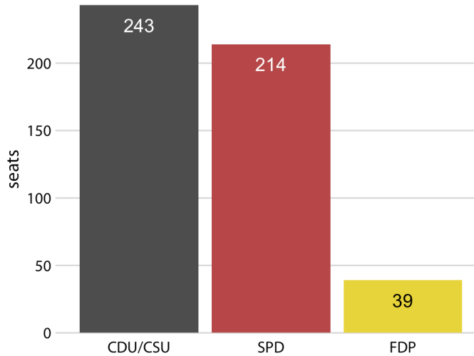
Figure 10-3. Party composition of the eighth German Bundestag, 1976–1980, visualized as side-by-side bars. As in Figure 10-2, it is not immediately obvious that SPD and FDP jointly had more seats than CDU/CSU. Data source: Wikipedia.
