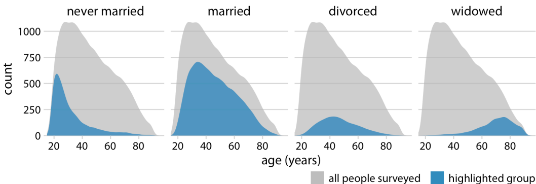
Figure 10-11. Marital status by age, shown as proportion of the total number of people in the survey. The colored areas show the density estimates of the ages of people with the respective marital status, and the gray areas show the overall age distribution. Data source: GSS.
