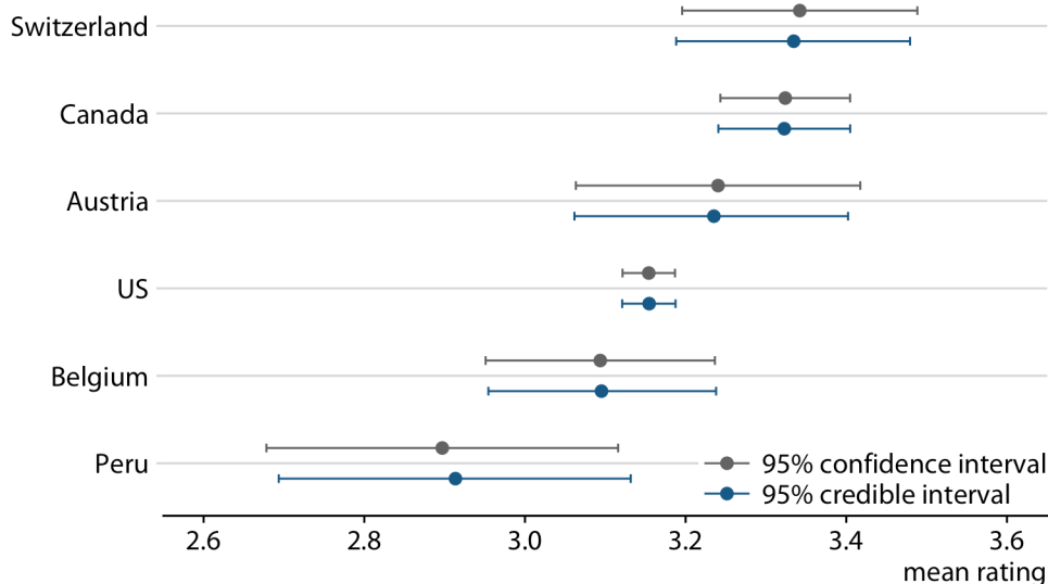
Figure 16-13. Comparison of frequentist confidence intervals and Bayesian credible intervals for mean chocolate ratings. We see that the two approaches yield similar but not exactly identical results. In particular, the Bayesian estimates display a small amount of shrinkage, which is an adjustment of the most extreme parameter estimates toward the overall mean. (Note how the Bayesian estimate for Switzerland is slightly moved to the left and the Bayesian estimate for Peru is slightly moved to the right relative to the respective frequentist estimates.) The frequentist estimates and confidence intervals shown here are identical to the results for 95% confidence shown in Figure 16-7. Data source: Brady Brelinski, Manhattan Chocolate Society.
