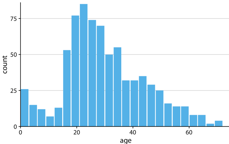
Figure 25-2. Histogram of the ages of Titanic passengers. This is the same histogram as in Figure 25-1, now drawn with filled bars. The shape of the age distribution is much more easily discernible in this variation of the figure. Data source: Encyclopedia Titanica.
