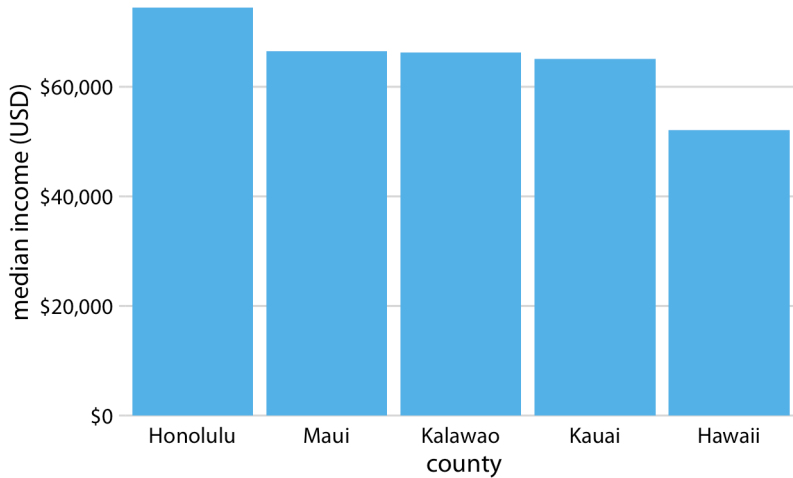
Figure 17-2. Median income in the five counties of the state of Hawaii. Here, the y -axis scale starts at $0 and therefore the relative magnitudes of the median incomes in the five counties are accurately shown. Data source: 2015 Five-Year American Community Survey.
