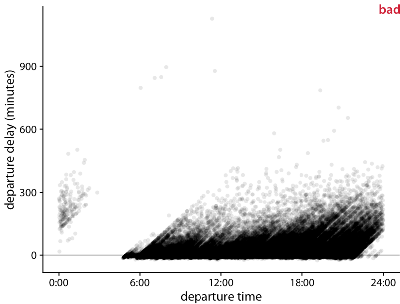
Figure 18-5. Departure delay in minutes versus flight departure time, for all flights departing Newark Airport (EWR) in 2013. Each dot represents one departure. Data source: US Dept. of Transportation, Bureau of Transportation Statistics.
