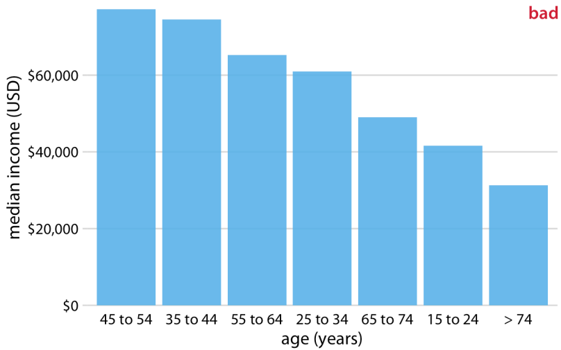
Figure 6-6. 2016 median US annual household income versus age group, sorted by income. While this order of bars looks visually appealing, the order of the age groups is now confusing. Data source: US Census Bureau.
