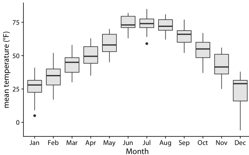
Figure 25-9. Distributions of daily mean temperatures in Lincoln, NE, in 2016. By giving the boxes a light gray shading, we can make them stand out better against the background. Data source: Weather Underground.
