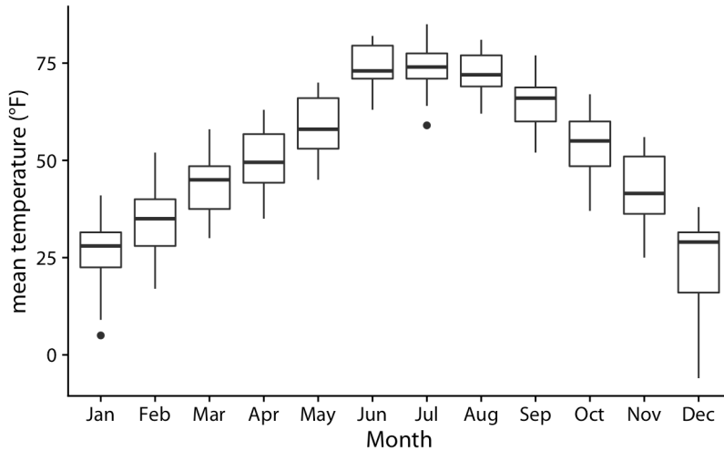
Figure 25-8. Distributions of daily mean temperatures in Lincoln, NE, in 2016. Boxes are drawn in the traditional way, without shading. Data source: Weather Underground.
