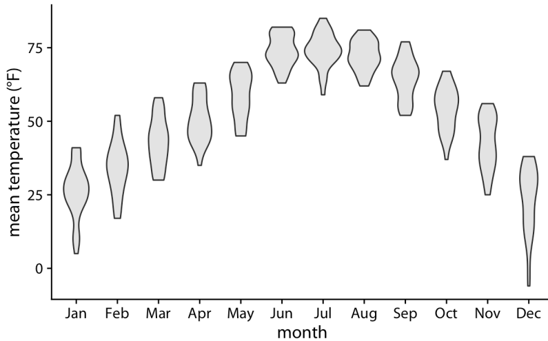
Figure 9-5. Mean daily temperatures in Lincoln, NE, visualized as violin plots. Data source: Weather Underground.
