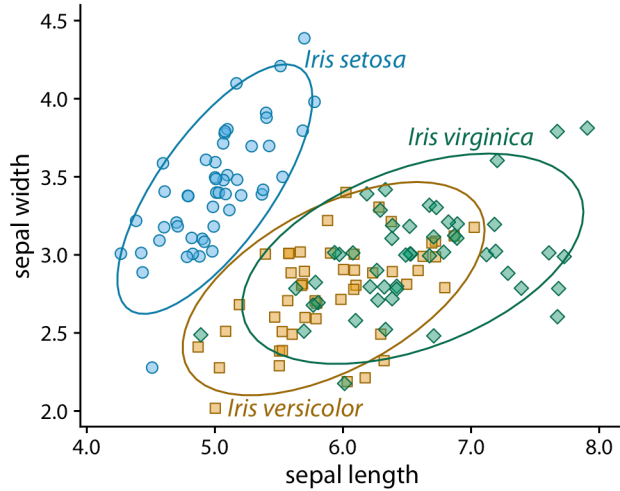
Figure 20-9. Sepal width versus sepal length for three different Iris species. The points representing different Iris species have been directly labeled with colored ellipses and text labels. Compared to Figure 20-3, I have removed the background grid here because the figure was becoming too busy. Data source: [Fisher 1936].
