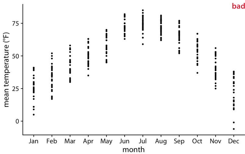
Figure 9-6. Mean daily temperatures in Lincoln, NE, visualized as strip charts. Each point represents the mean temperature for one day. This figure is labeled as “bad” because so many points are plotted on top of each other that it is not possible to ascertain which temperatures were the most common in each month. Data source: Weather Underground.
