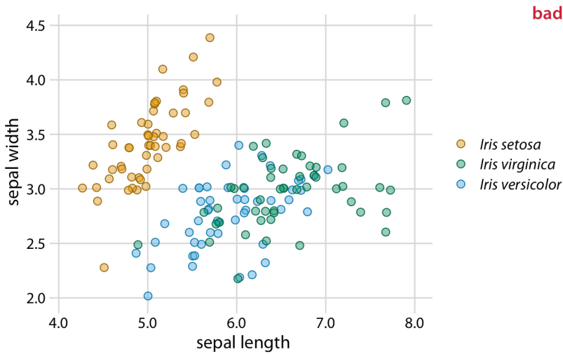
Figure 20-1. Sepal width versus sepal length for three different Iris species ( Iris setosa , Iris virginica , and Iris versicolor ). Each point represents the measurements for one plant sample. A small amount of jitter has been applied to all point positions to prevent overplotting. The figure is labeled “bad” because the virginica points in green and the versicolor points in blue are difficult to distinguish from each other. Data source: [Fisher 1936].
