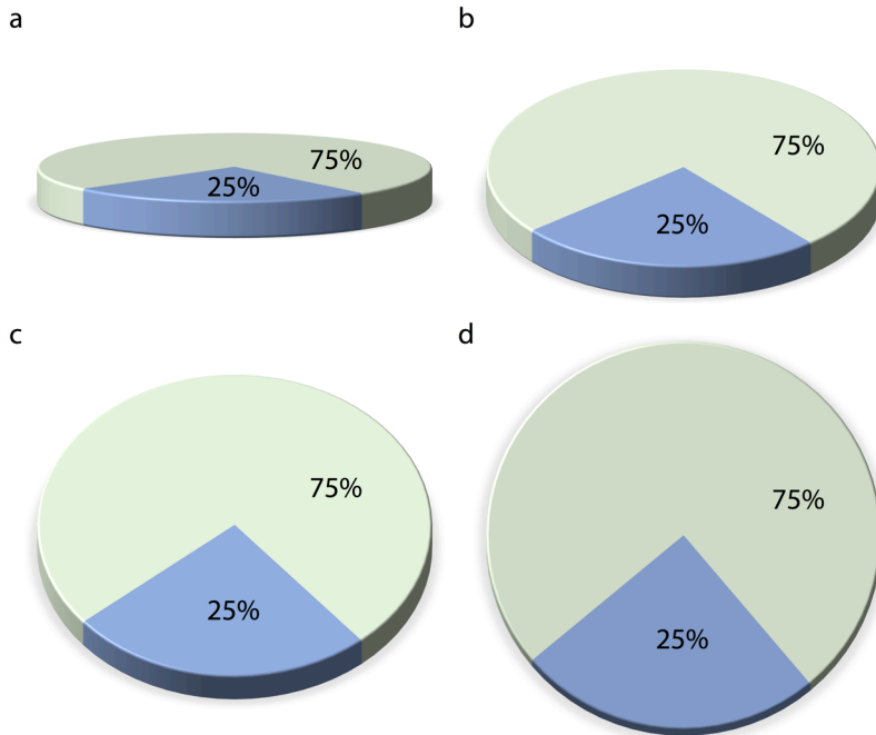
Figure 26-1. The same 3D pie chart shown from four different angles. Rotating a pie into the third dimension makes pie slices in the front appear larger than they really are and pie slices in the back appear smaller. Here, in parts (a), (b), and (c), the blue slice corresponding to 25% of the data visually occupies more than 25% of the area representing the pie. Only part (d) is an accurate representation of the data.
