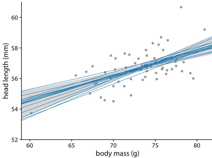
Figure 16-16. Head length versus body mass for male blue jays. In contrast to Figure 16-15, the straight blue lines now represent equally likely alternative fits randomly drawn from the posterior distribution. Data source: Keith Tarvin, Oberlin College.
