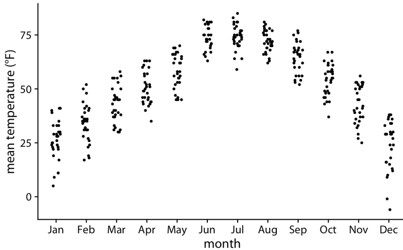
Figure 9-7. Mean daily temperatures in Lincoln, NE, visualized as strip charts. The points have been jittered along the x axis to better show the density of points at each temperature value. Data source: Weather Underground.
