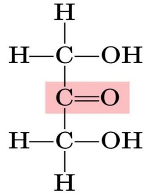
Dihydroxyacetone, a ketotriose
