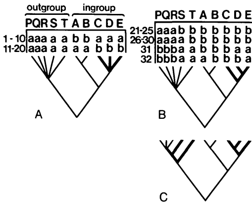
FIG. 14. Another data set of 32 characters with states a and b distributed as shown. (A) Characters 1-20 partially resolve the ingroup. (B and C) Characters 21-32 resolve the ingroup further. Simultaneously resolving the outgroup and the ingroup gives more parsimonious cladogram (C) than assuming the most common state within the outgroup to be ancestral (B). If T were the only outgroup terminal taxon, finding the unrooted network for the ingroup alone then attaching T would give a less than most parsimonious cladogram.
