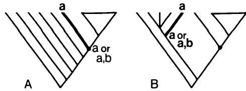
FIG. 8. The importance of (A) the first outgroup and (B) the basalmost member of a heterogeneous outgroup (Rule 3).
