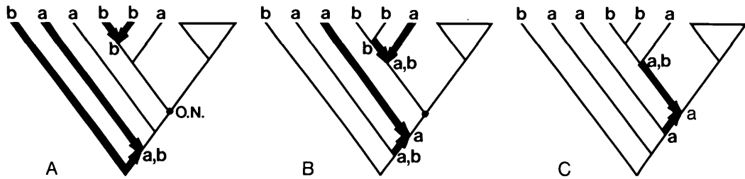
FIG. 4. An application of the outgroup algorithm for binary characters. The internal nodes are labelled, starting at the outgroup terminal taxa and proceeding toward the outgroup node (O.N.).
