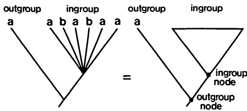
FIG. 1. Terms and symbols used throughout the paper. The unresolved ingroup is shown as a triangle. There may be more than one outgroup.
