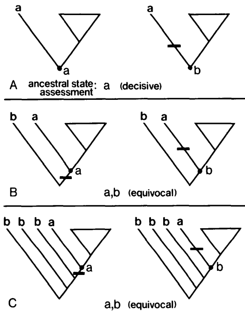
FIG. 3. The use of parsimony to assess the state at the outgroup node. Ancestral state assessment shown below each example. (A) State a requires no steps and, hence, is more parsimonious than state b . (B and C) a and b are equally parsimonious.
