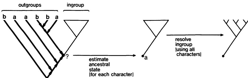
FIG. 2. Two-step cladistic analysis. First, the ancestral states (at the outgroup node) are estimated using the outgroups and parsimony. Second, the most parsimonious ingroup cladogram is sought.
