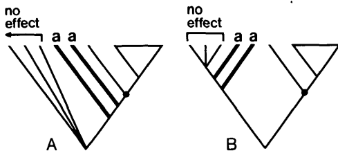
FIG. 6. The buffering effect of doublets. Groups beyond the doublet have no effect on the polarity assessment (Rule 1 of "Uncertain Outgroup Relationships").
