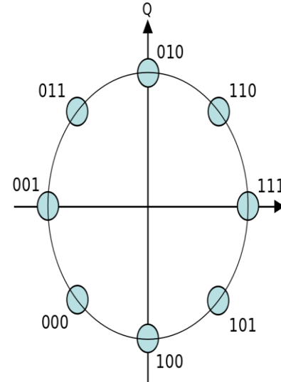
8-PSK
