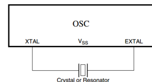
Figure 25-2. Crystal/Ceramic Resonator Connections - Connection 1
