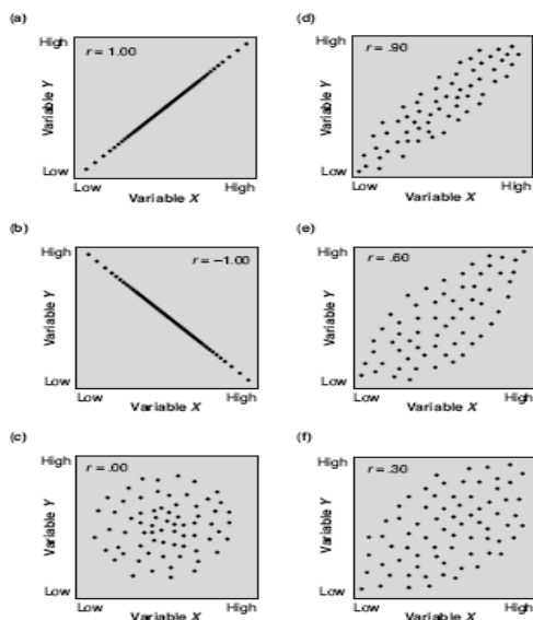
FIGURE 9 Scatterplot of Different Correlation Coefficients. Source: Hopkins, Kenneth, Educational and Psychological Measurement and Evaluation , 8th ©1998. Printed and Electronically reproduced by permission of Pearson Education, Inc., Upper Saddle River, New Jersey.
