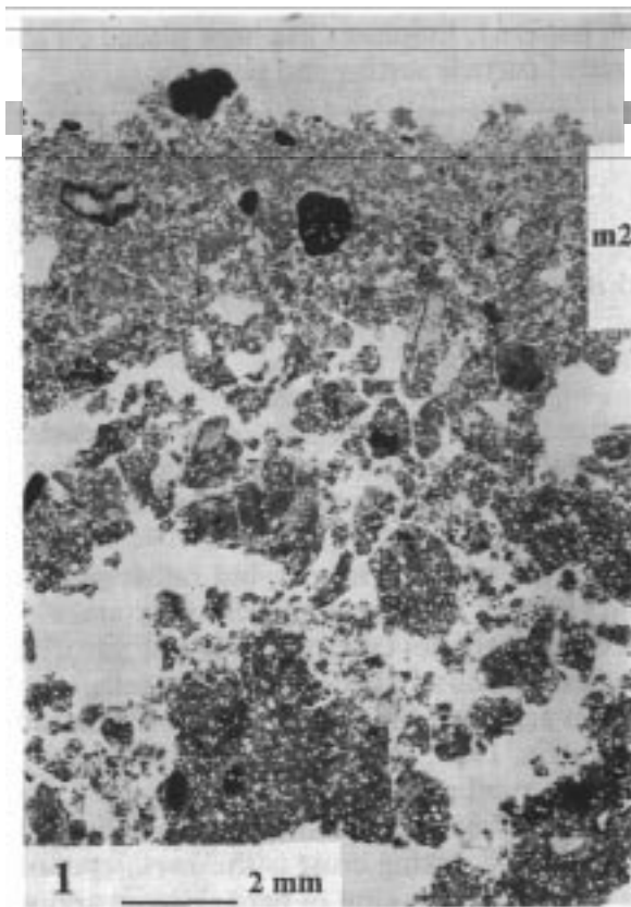
Photo 1. Slaking structural crust on a loamy soil (vertical thin section, plain light): thin, apedal layer (m2), without any clear textural disjunction.
