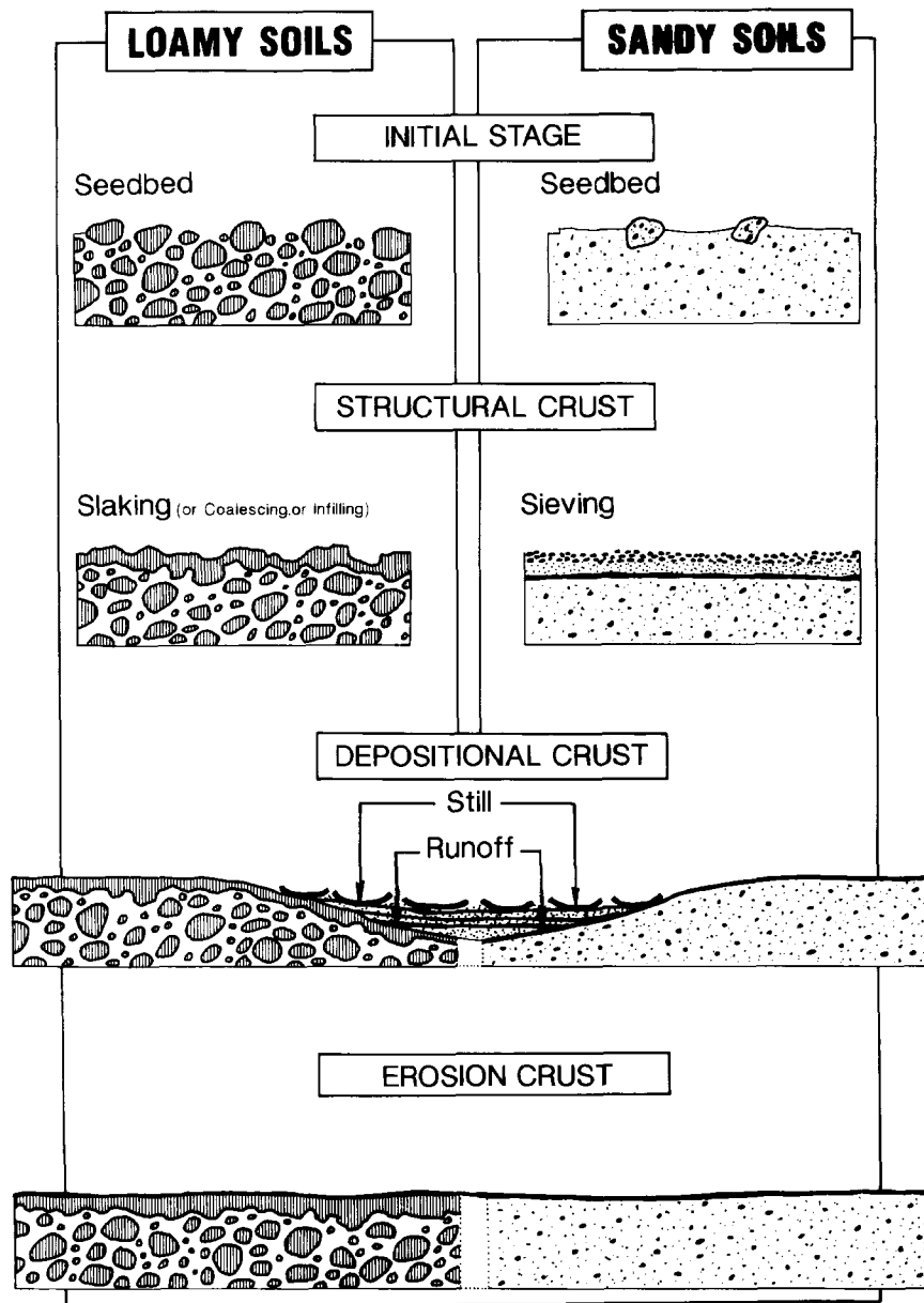
Fig. 2. Diagrammatic representation of the time-sequence soil crusts in loamy and sandy soils.
