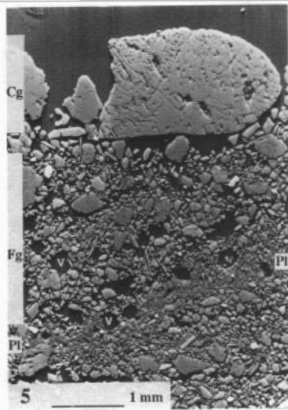
Photo 5. Sieving structural crust on a sandy soil (vertical polished section, BESI mode): three-layered crust with loose coarse grains at the top ( Cg ), fine, densely packed grains and vesicular voids ( v ) in the middle ( Fg ), and a plasmic layer ( Pl ) at the bottom.
