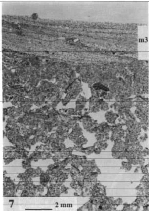
Photo 7. Runoff depositional crust on a loamy cultivated soil (vertical thin section, plain light): microbedded layer with submillimetric moderately sorted microbeds ( m3 ), overlying a previously-formed structural crust.
