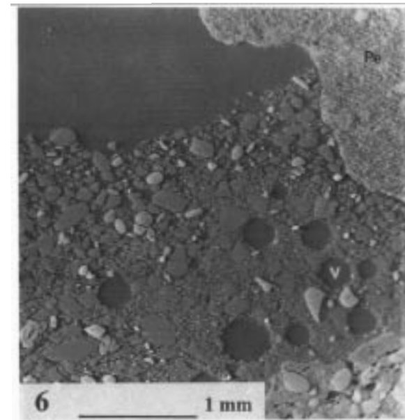
Photo 6. Sieving structural crust on a sandy soil (vertical polished section, BESI mode): pavement crust, consisting of coarse fragments ( Pe ) embedded in a sieving crust with a pronounced vesicular porosity, especially under the pebbles ( v ).
