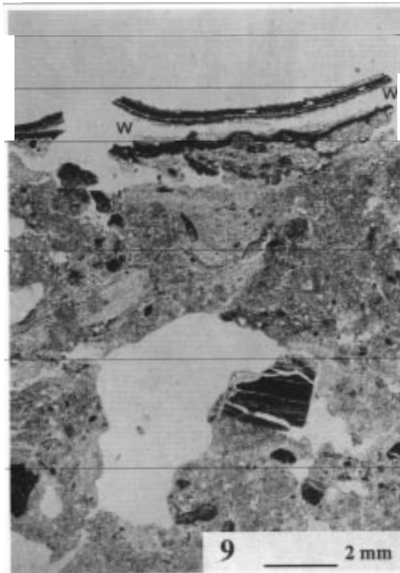
Photo 9. Still depositional crust on a loamy soil (vertical thin section, plain light): well-sorted layer ( W ), broken up into curled-up plates due to drying, and overlying a structural crust.
