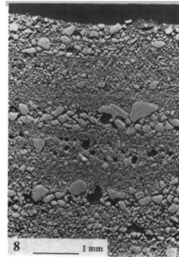
Photo 8. Runoff depositional crust on a sandy soil (vertical polished section, BES mode): submillimetric microbeds exhibiting various mean particle sizes and sorting.
