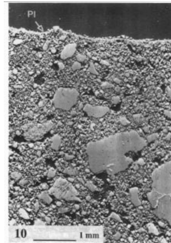
Photo 10. Erosion crust on a sandy soil (vertical polished section, BES mode): thin and smooth plasmic layer ( PI ).
