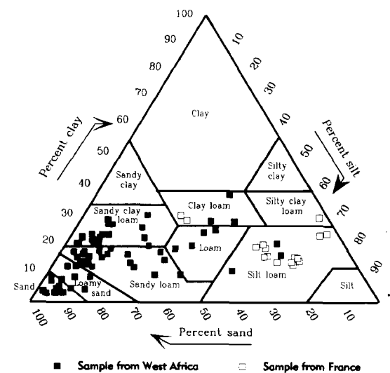
Fig. 1. Texture of the studied samples.
