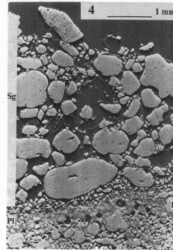
Photo 4. Sieving structural crust on a sandy soil (vertical polished section, BES mode): two-layered crust, made up of a layer of loose skeleton grains ( Sg ) overlying a plasmic layer ( Pl ).
