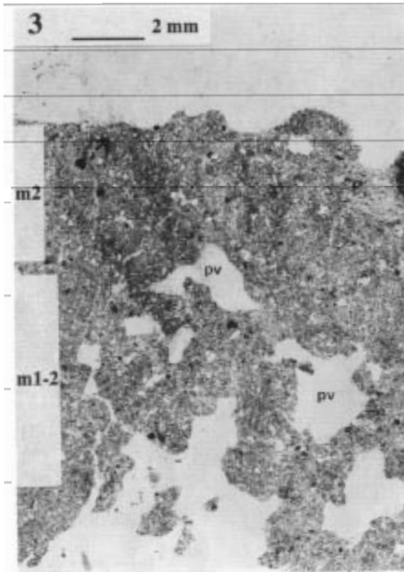
Photo 3. Coalescing structural crust on a loamy soil (vertical thin section, plain light): apedal layer with isolated pores ( m2 ), overlying a compacted layer ( m1-2 ) with convexo-concave packing voids ( pv ).
