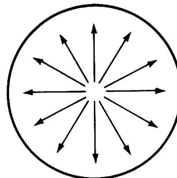
TM_{01}
