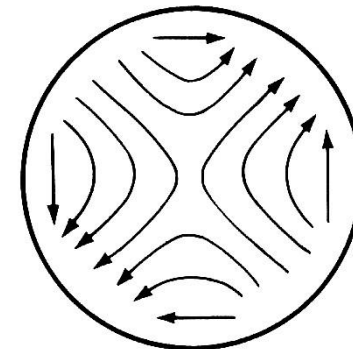
HE_{21}
