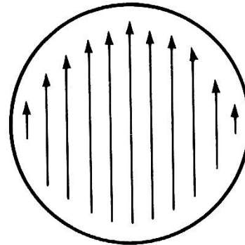
HE_{11}
