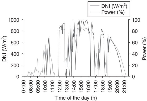
9.25 Daily power output of a grid-connected Dish Stirling system with unfavourable irradiation.
