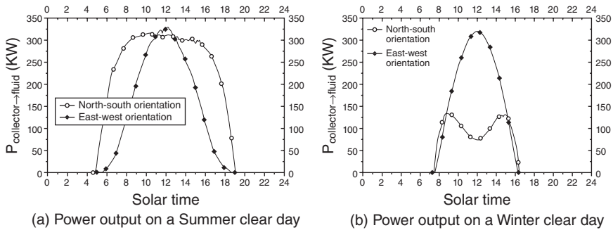
7.16 Daily thermal output of a EuroTrough-100 parabolic-trough collector located in Southern Spain, on a Summer (a) and Winter (b) clear day, and with two different orientations of its axis (north-south and east-west).
