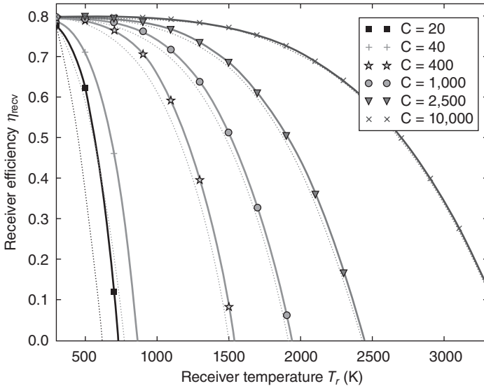
2.15 Efficiency of a simplified solar collector with 100% optical efficiency, average absorptivity of 0.8 (assumed equal to emissivity) plotted both with no external convective loss (solid lines) and with 20 \text{ W/m}^2\text{K} external convective loss (dotted lines). DNI is 800 \text{ W/m}^2 , ambient temperature 300 \text{ K} , and sky temperature 270 \text{ K} .
