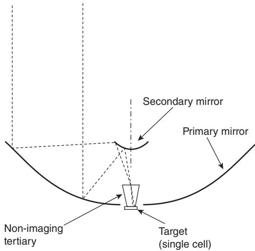
10.11 Cross section, reflective cassegrainean concentrator coupled to a non-imaging tertiary.
