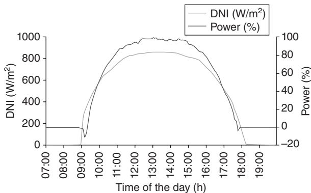
9.23 Daily power output of a grid-connected dish Stirling system with favourable irradiation.
