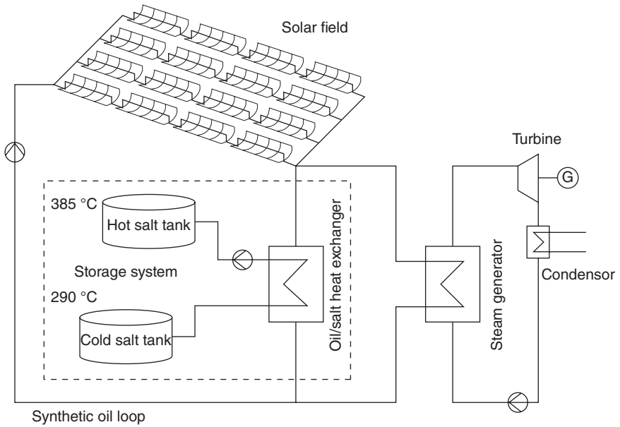
11.5 Simplified scheme of a parabolic trough plant using thermal oil as HTF with an indirect two-tank molten salt storage concept.
