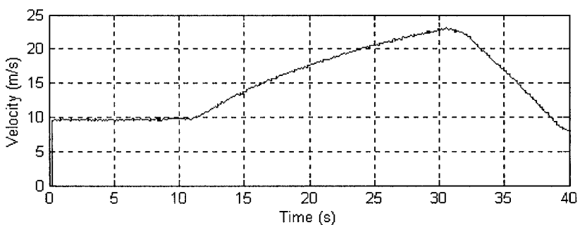
Figure 14-7. Acceleration starting at 20mph on dry concrete surface
