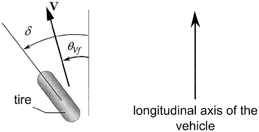
Figure 2-7. Tire slip-angle
