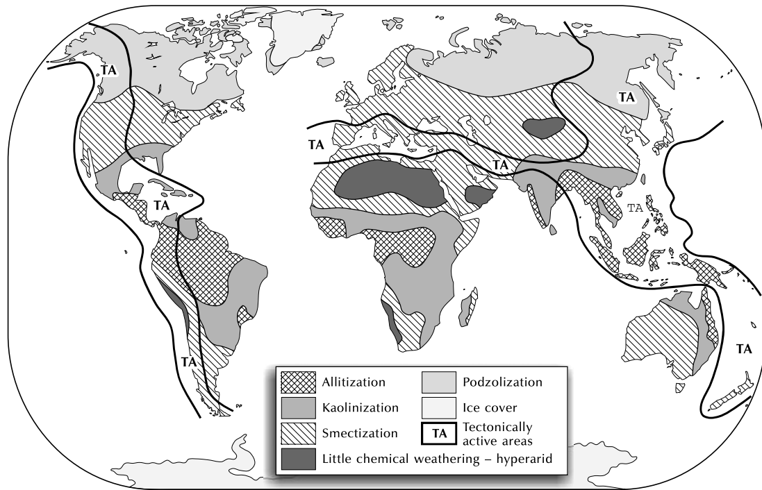
Figure 6.4 The main weathering zones of the Earth. Source: Adapted from Thomas (1974, 5)
