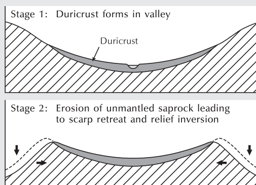
Figure 6.2 Development of inverted relief associated with duricrust formation.
