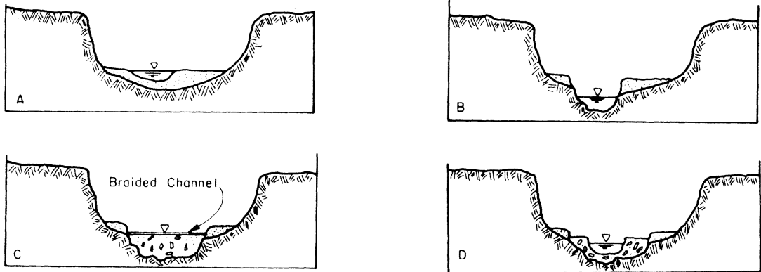
FIGURE 6. Diagrammatic cross sections of experimental channel 1.5 m from outlet of drainage system (base level) showing reponse of channel to one lowering of base level.
