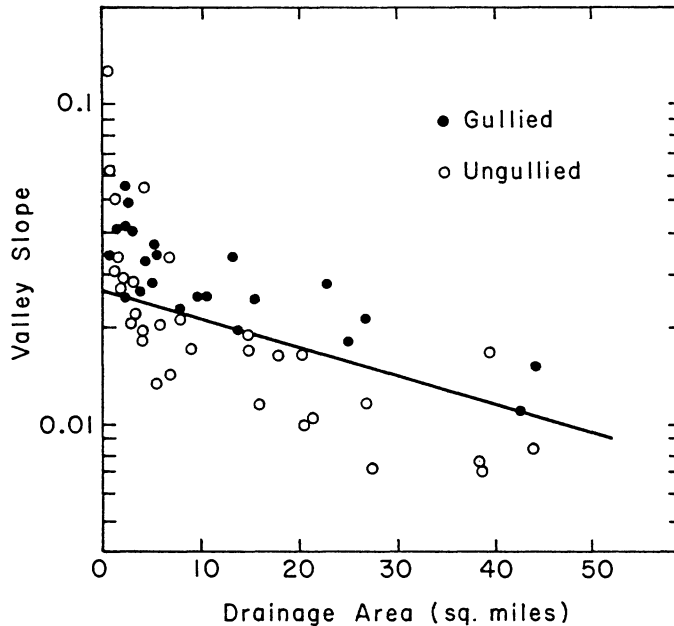
FIGURE 1. Relation between valley slope and drainage area, Piceance Creek Basin, Colorado. Line defines threshold slope that separates gullied from ungullied valley floor. (FROM PATTON AND SCHUMM, 1975)
