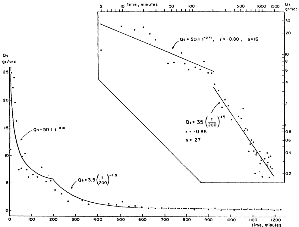
FIGURE 8. Effects of development of armours on sediment discharge, Q_s , during experimental study of gully erosion. At about 200 minutes into the run the armour became effective and abruptly reduced sediment discharge. The change is displayed very clearly in the logarithmic plot
