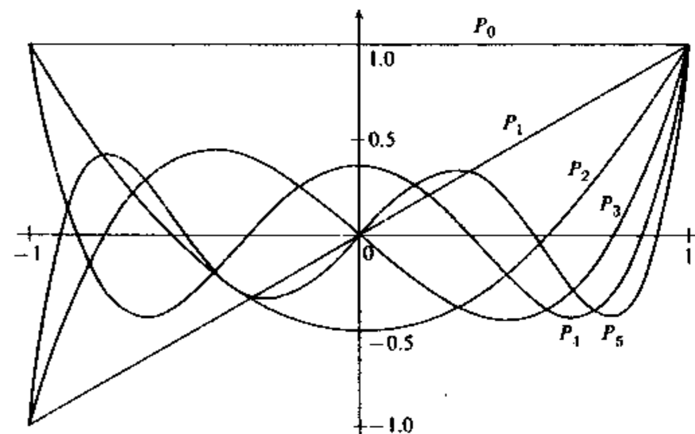
Legendre polynomials
