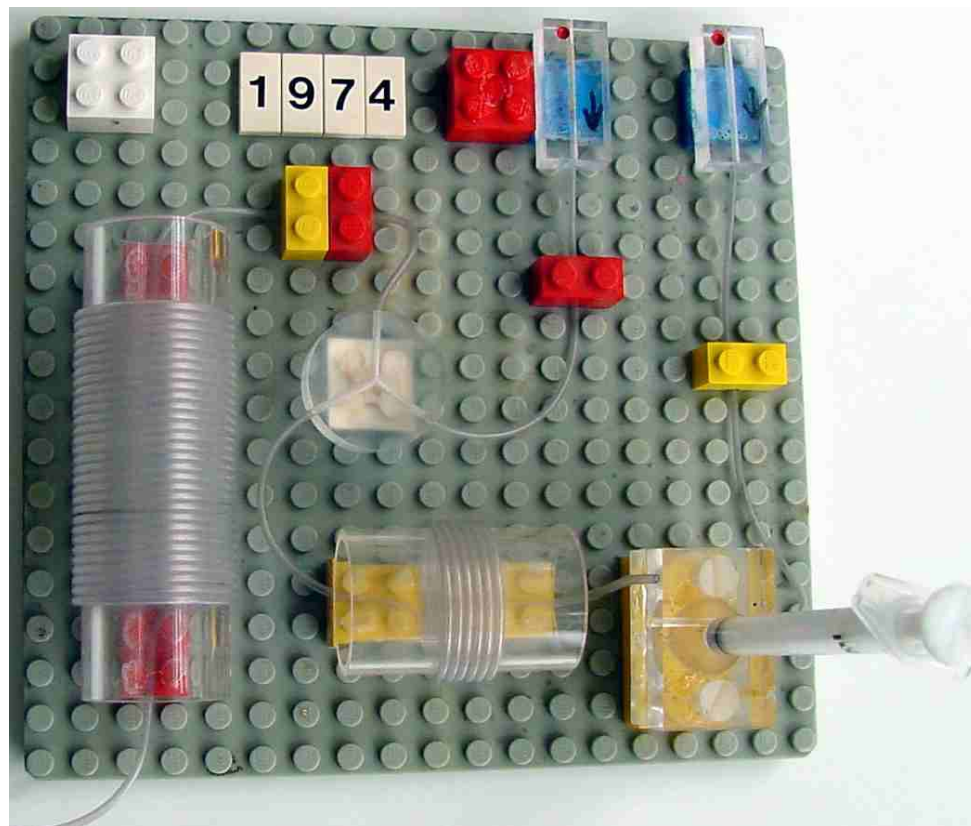
Two reagents, confluence point
