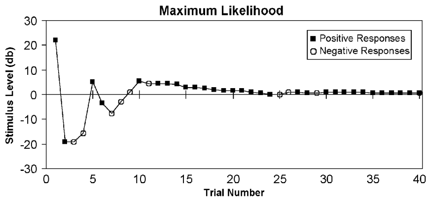
Figure 3. Adaptive track following a maximum-likelihood adaptive procedure, as developed by Green (1993). Decibel values are relative to the arbitrary threshold of 0 dB.
