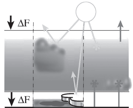
Fig. 1. Solar shortwave (yellow) and infrared longwave (red) radiation in the atmosphere. Fluxes ending in arrows are transmitted; fluxes ending in stars are absorbed. (left section) Global warming-independent adjustment to forcing eliminates net atmospheric energy absorption. Hence, net forcing ( \Delta F ) is the same at the tropopause and surface. (middle section) Reflection of sunlight by clouds and the surface affects precipitation indirectly through surface temperature. (right section) Atmospheric absorption of sunlight and absorption and emission of infrared affect precipitation through surface temperature and directly through the tropospheric energy budget. Original color image appears at the back of this volume.
