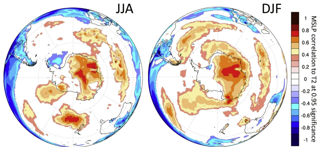
Fig. 4. Correlation between JJA and DJF MSLP compared to JJA and DJF T2 (1979–2015) using ERAI. All filled contours are at or above 95% significance (derived using a Pearson's r significance threshold for the given sample size).
