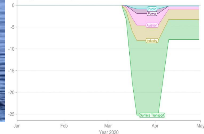
Change in daily fossil CO 2 emissions, % Brazil (peak decrease -25%)
