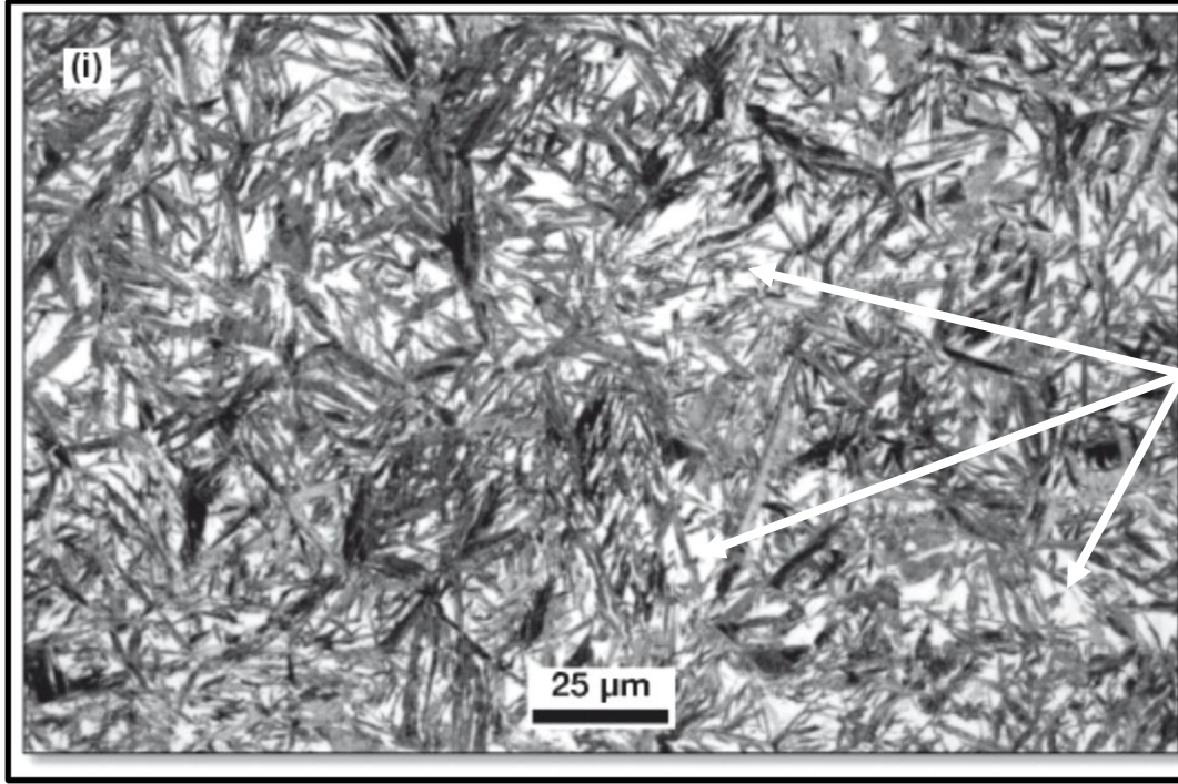
Figura 10.64(i) – AISI 43100 – 200°C
