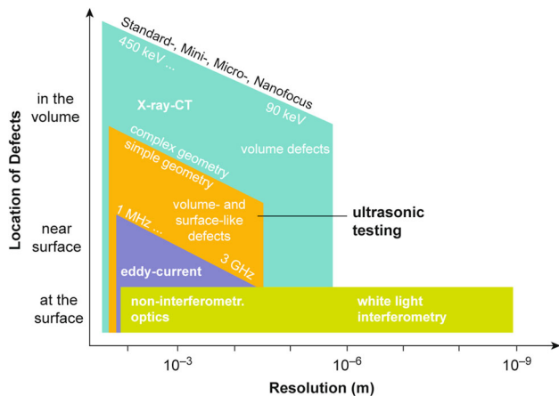
Fig. 4. Classification and comparison of chosen NDT techniques and optical measurement techniques according to detectable defect location and spatial resolution. Reproduced with permission from Ref. 82.
