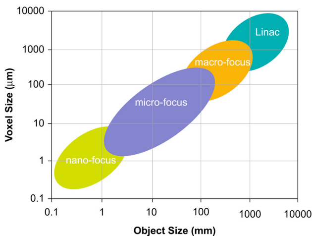
Fig. 5. Resolution versus object size limitations. Reproduced with permission from Ref. 93.
