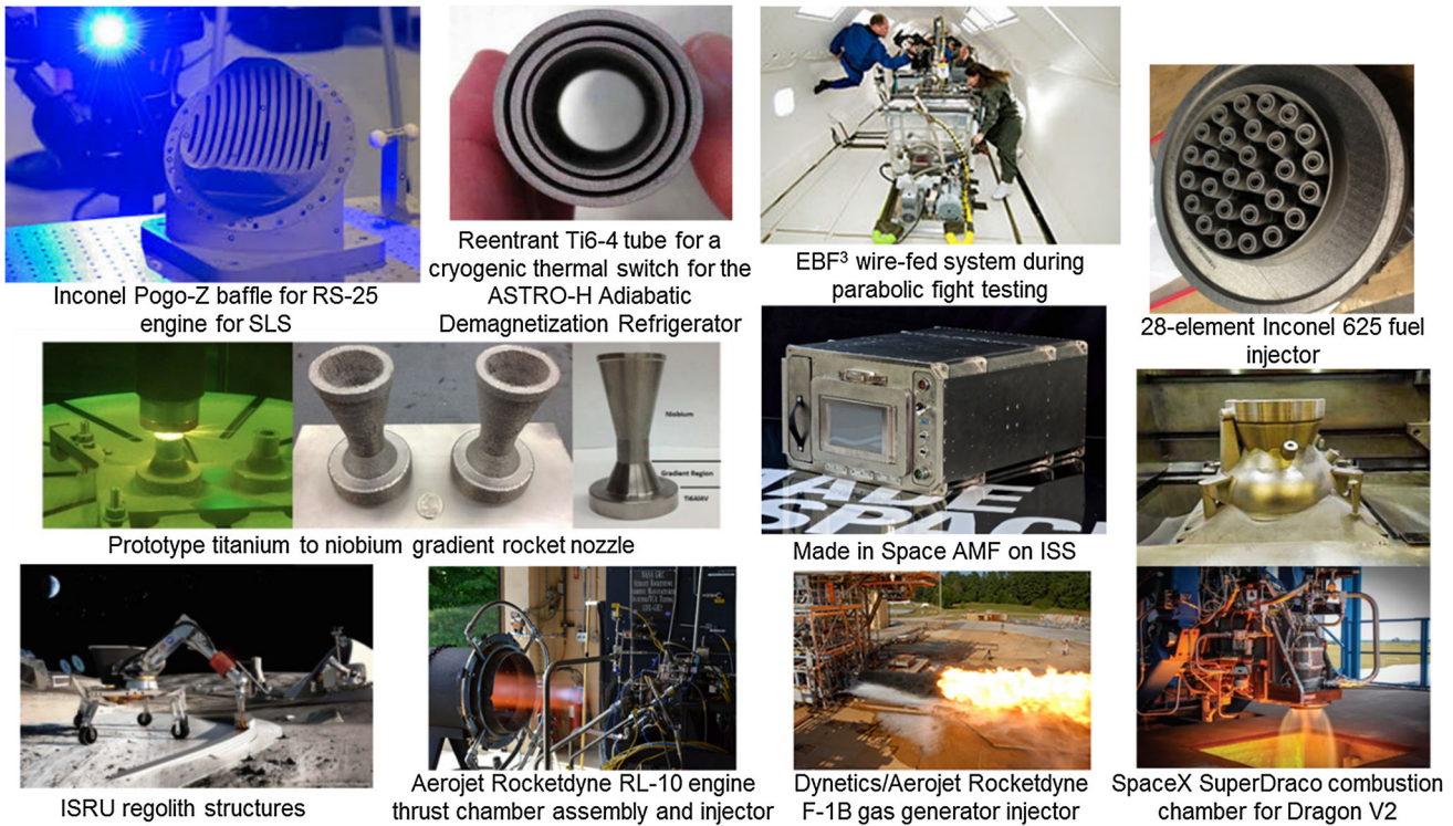
Fig. 6. Representative NASA agency and prime contractor additive manufacturing activities 96 .
