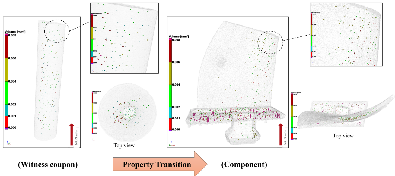
Fig. 3. XCT results conducted on a witness coupon and a component made at the same time demonstrating challenging property/characteristics transfer from witness coupon to the actual component. Color-coded dots exhibiting the presence of defects with various shapes, sizes and distribution. 78 3D visualization can be accessed on the online version of this paper.
