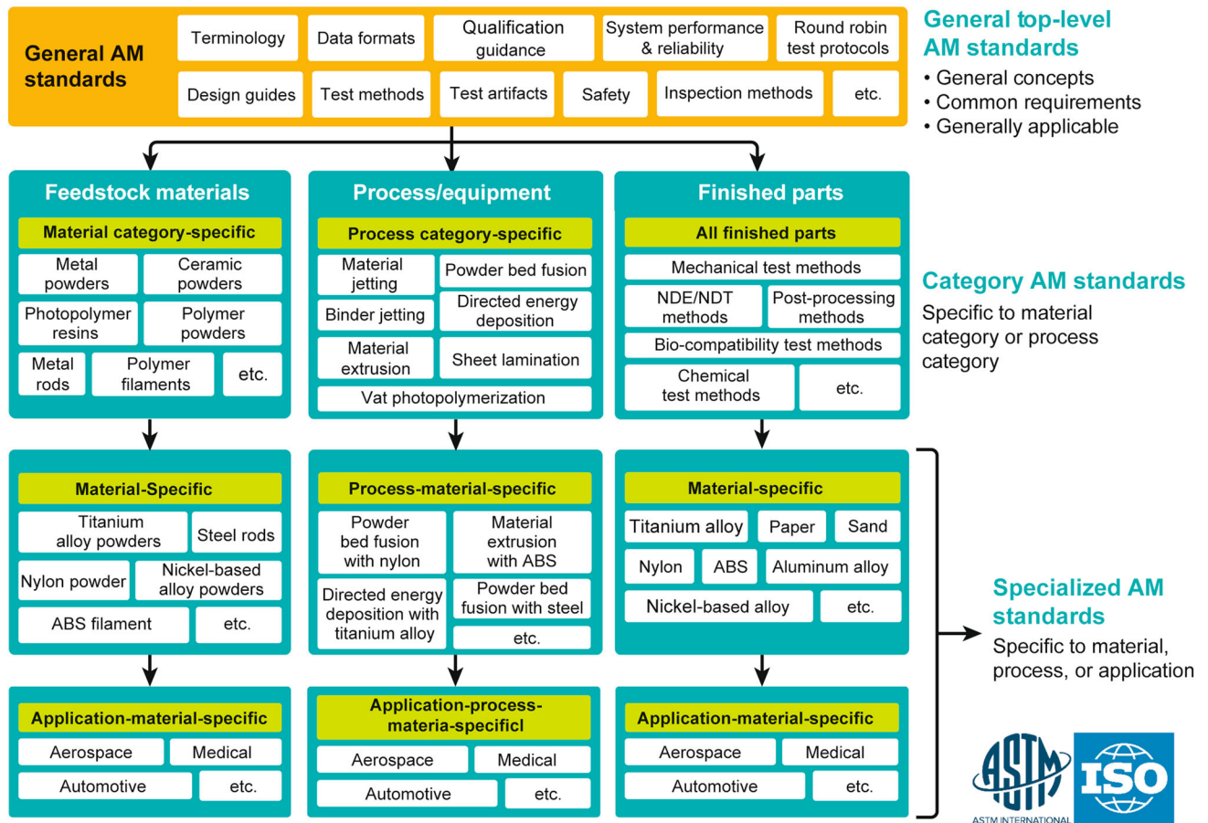
Fig. 7. Additive manufacturing standardization framework (developed and approved by ASTM F42/ISO TC261).
