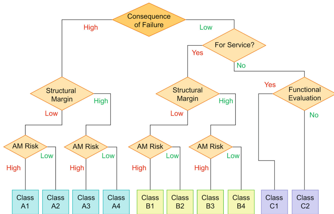
Fig. 1. AM parts classification. (adapted from Ref. 17 with permission).
