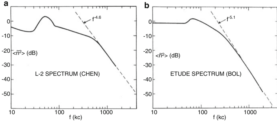
Fig. 8.38 Turbulence spectra in (a) the L-2, a reflex arc ( 2000 \text{ G}, 10^{12} \text{ cm}^{-3} ); and (b) the Etude, a stellarator ( 6700 \text{ G}, 10^{13} \text{ cm}^{-3} ). Here, frequency is measured rather than k
