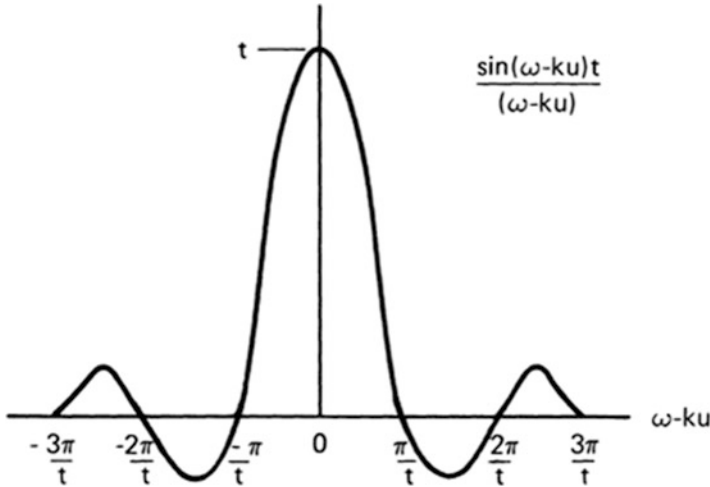
Fig. 7.25 A function which describes the relative contribution of various velocity groups to Landau damping
