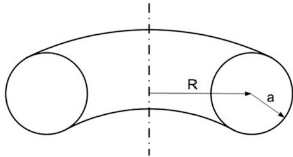
Fig. 10.19 Drawing of a tilt instability in an FRC
