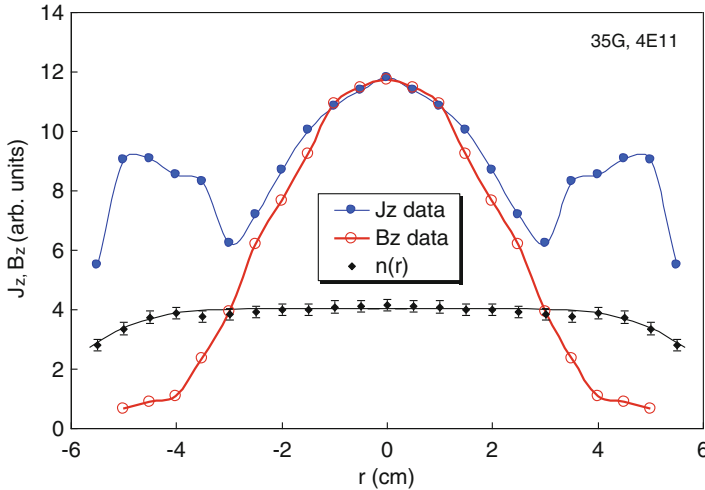
Fig. 9.13 Radial profiles of n(r) , B_z(r) , and J_z(r) in a helicon discharge at B = 3.5 mT and n = 4 \times 10^{17} \text{ m}^{-3} (D.D. Blackwell, T.G. Madziwa, D. Arnush, and F.F. Chen, Phys. Rev. Lett. 88 , 145002 (2002))
