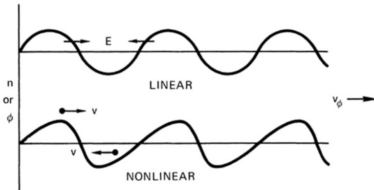
Fig. 8.9 A large-amplitude ion wave steepens so that the leading edge has a larger slope than the trailing edge
