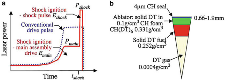
Fig. 10.63 (a) Time sequence of a shock ignition pulse, compared to a conventional pulse. The total time has to be short enough to avoid heating the hohlraum [L.J. Perkins et al., Phys. Rev. Lett. 103 , 045004 (2009)]. (b) Design of a capsule for shock ignition
