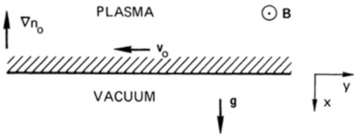
Fig. 6.10 A plasma surface subject to a gravitational instability
