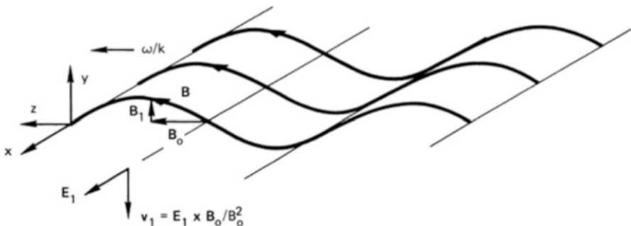
Fig. 4.46 Relation among the oscillating quantities in an Alfvén wave and the (exaggerated) distortion of the lines of force
