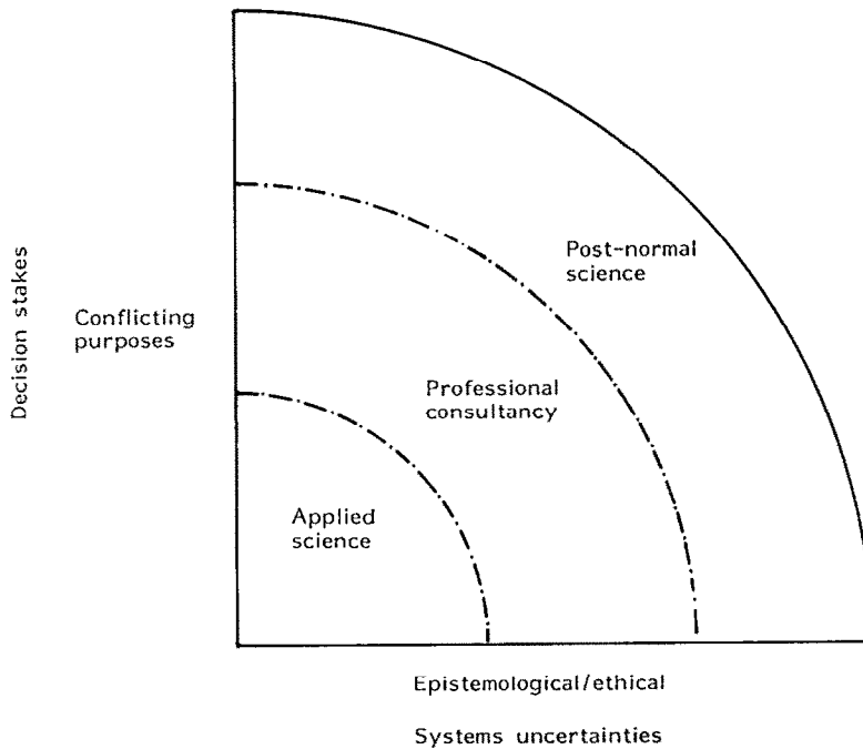
Figure 4. Post-normal science
