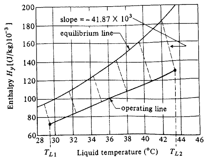
FIGURE 10.5-4. Graphical solution of Example 10.5-1.
