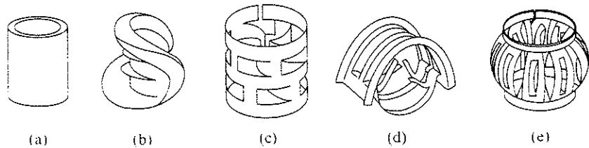
FIGURE 10.6-4. Typical random or dumped tower packings: (a) Raschig ring; (b) Berl saddle; (c) Pall ring; (d) Intalox metal, IMTP; (e) Jaeger Metal Tri-Pack.
