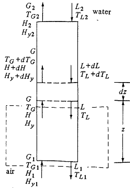
FIGURE 10.5-2. Continuous countercurrent adiabatic water cooling.
