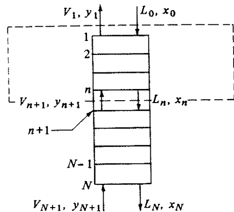
FIGURE 10.6-7. Material balance in an absorption tray tower.
