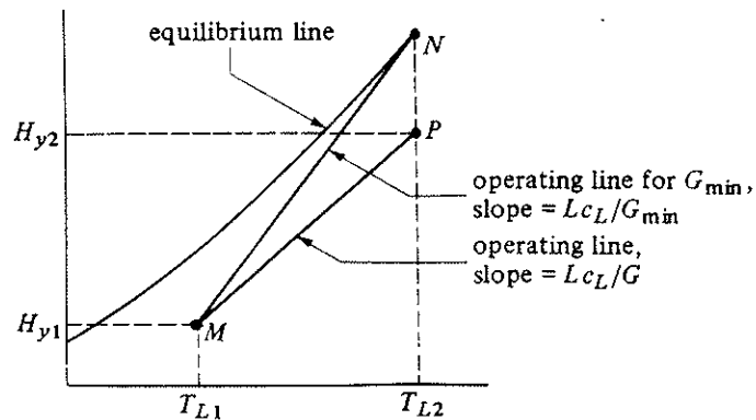
FIGURE 10.5-5. Operating-line construction for minimum gas flow.
