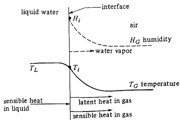
FIGURE 10.5-1. Temperature and concentration profiles in upper part of cooling tower.
