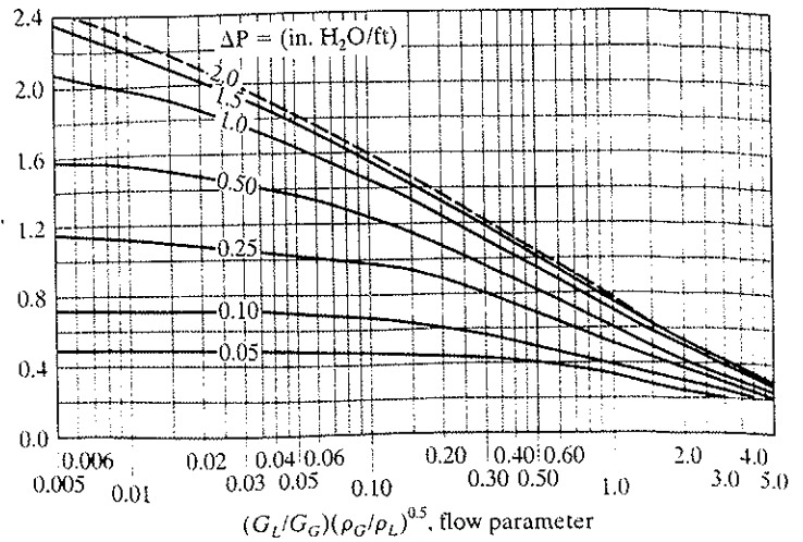
FIGURE 10.6-5. Pressure-drop correlation for random packings by Strigle. (From R. F. Strigle, Jr., Random Packings and Packed Towers . Houston: Gulf Publishing Company, 1987. With permission from Elsevier Science.)
