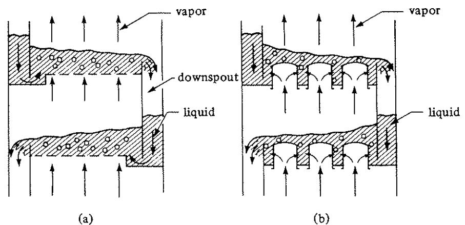
FIGURE 10.6-1. Tray contacting devices: (a) detail of sieve-tray tower, (b) detail of valve-tray tower.
