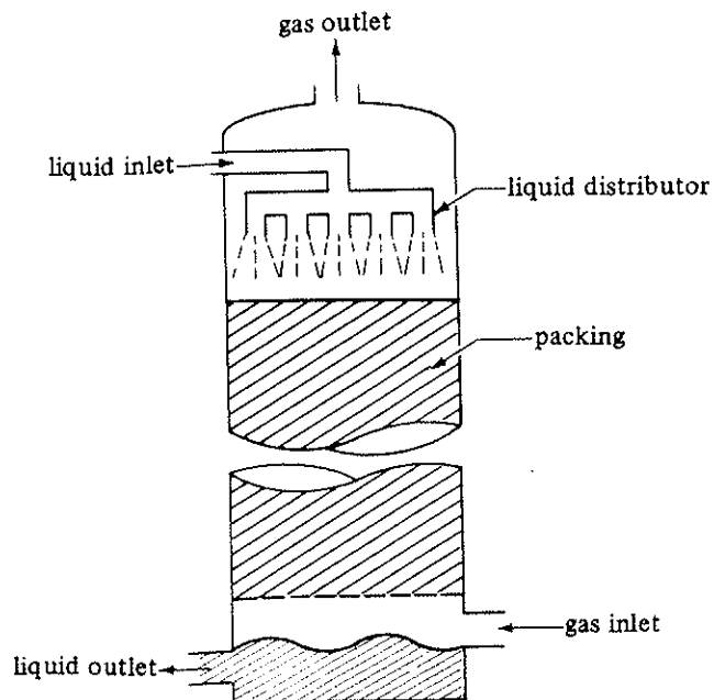
FIGURE 10.6-3. Packed tower flows and characteristics for absorption.
