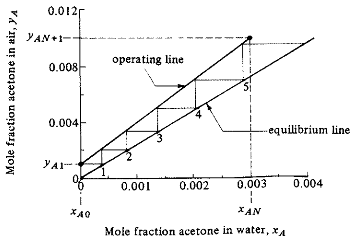
FIGURE 10.3-4. Theoretical stages for countercurrent absorption in Example 10.3-2.
