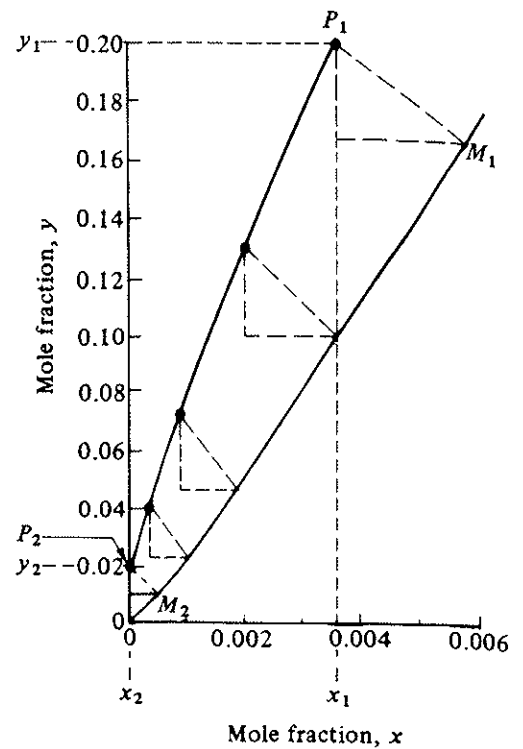
FIGURE 10.7-1. Operating line and interface compositions for Example 10.7-1.
