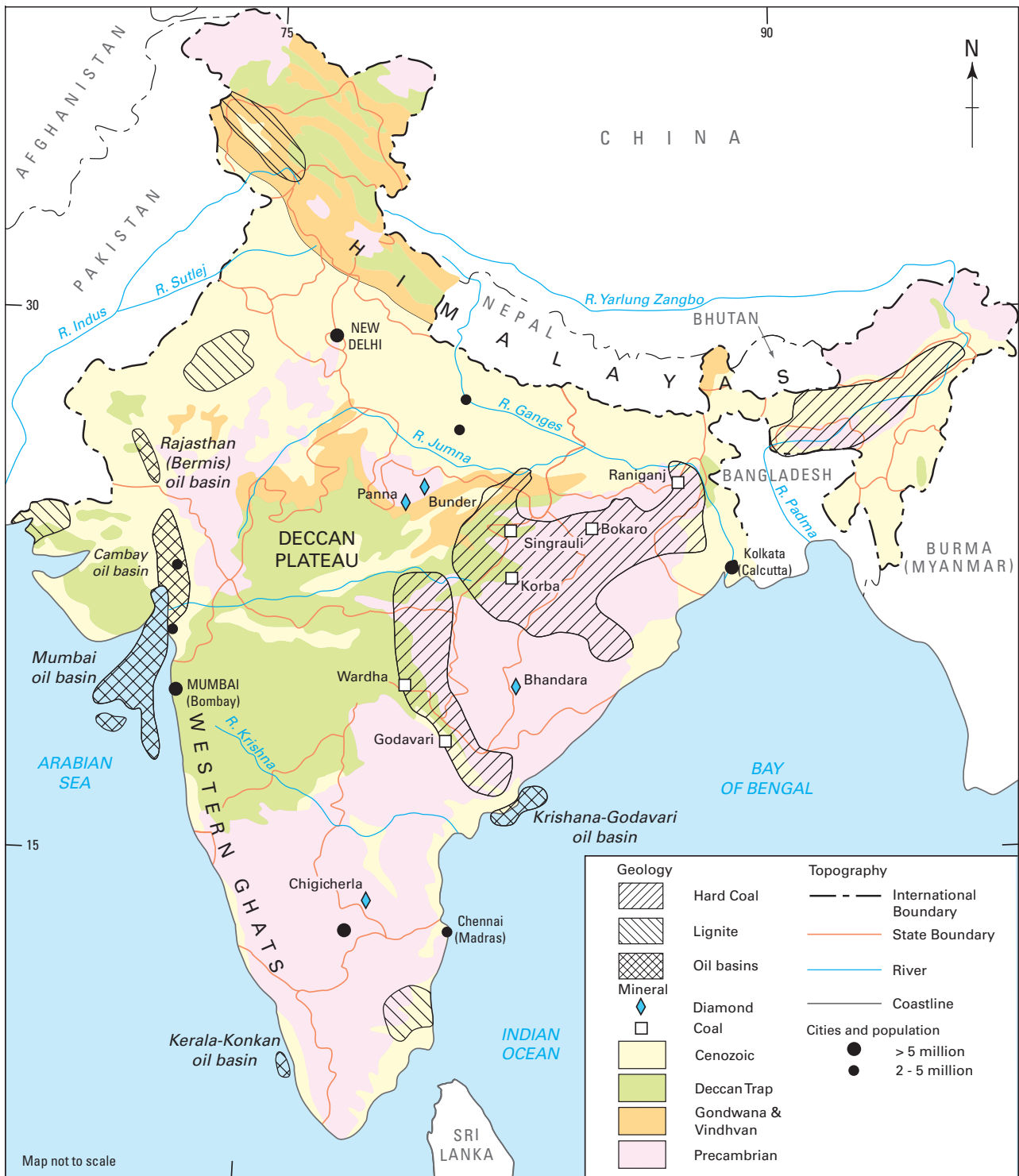
Figure 23 Selected major mines and important deposits in India (non-metallics).
