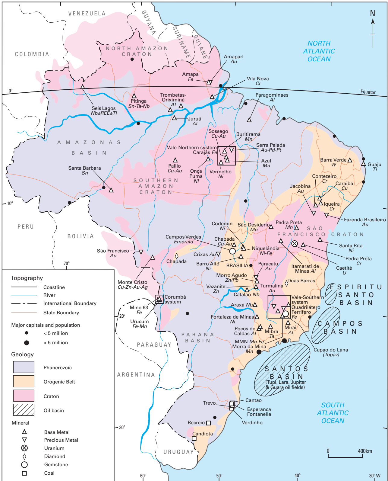
Figure 3 Selected major mines and important mineral deposits in Brazil.
