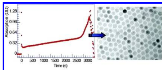
Figure 29. UV-vis spectra for the oxidation of Fe(CO) 5 by mCPBA showing burst nucleation. Reprinted with permission from ref 92. Copyright 2006 American Chemical Society.
