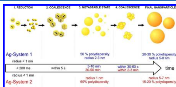
Figure 23. Schematic illustration of the deduced four-step growth mechanism of both silver nanoparticle systems. Reprinted with permission from ref 86. Copyright 2012 American Chemical Society.
