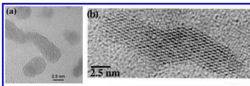
Figure 7. (a) Coalescence of platinum crystallites has led to this platinum nanowire. (b) A formation of four titania crystallites forming one large crystallite through orientated attachment. Reproduced with permission from ref 48. Copyright 1999 Elsevier.
