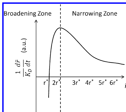
Figure 5. Schematic of [d\bar{r}/dt]/K_D as a function of \bar{r} for diffusion-controlled growth within an infinite diffusion layer showing how above 2r^* the size distribution narrows within increasing size.
