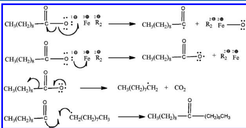
Figure 28. Example schematic for the formation of iron oxide through a radical in nonaqueous solutions. Reproduced from ref 91 with permission of the PCCP Owner Societies.
