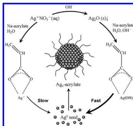
Figure 22. Mechanism for the formation of silver nanoparticles. Reproduced from ref 82 with permission of the PCCP Owner Societies.
