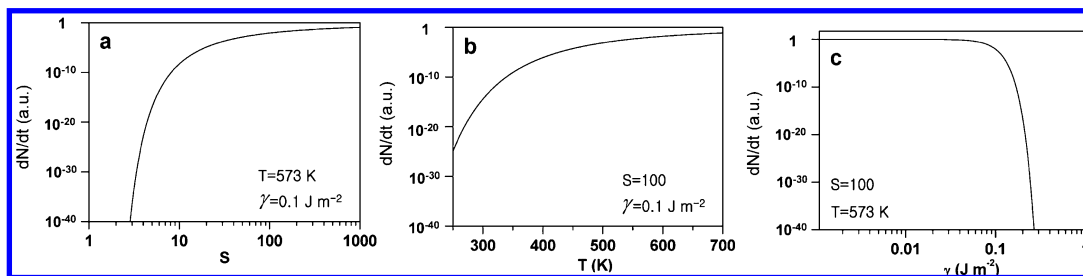
Figure 2. Nucleation rate as a function of a) supersaturation, b) temperature, and c) the surface free energy calculated using eq 6. v is set as 3.29 \times 10^{-5} \text{ m}^3 \text{ mol}^{-1} , the value for CdSe. The nucleation rate is normalized with the pre-exponential factor A . Reprinted with permission from ref 25. Copyright 2011 WILEY-VCH Verlag GmbH & Co. KGaA, Weinheim.
