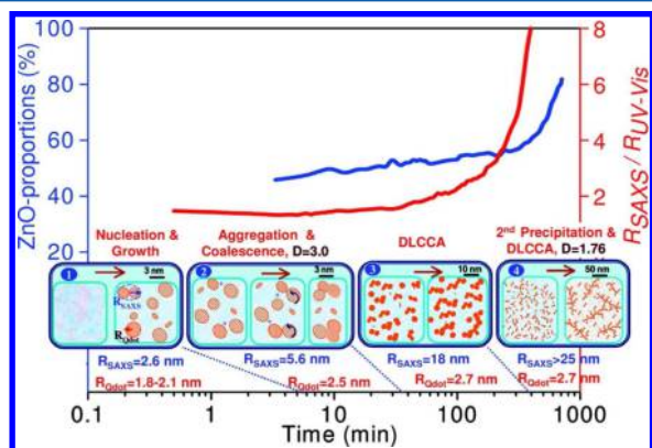
Figure 35. Schematic evolution of colloidal system as derived from the time evolution of the fractions of precursor and zinc oxide (XAFS), the quantum dot radius R_{UV-vis} and the aggregate of gyration radius R_g (SAXS). Reprinted with permission from ref 96. Copyright 2011 American Chemical Society.
