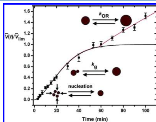
Figure 18. Plot of the growth of particle size with time showing the graph for a sigmoidal curve using V_{lim} is the mean volume at the end of coalescent growth before Ostwald ripening takes over in the linear region. Reprinted with permission from ref 74. Copyright 2010 American Chemical Society.
