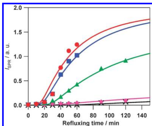
Figure 20. Time evolution of surface plasmon resonance intensity for the cases of x = 0 ( \times ), 0.4 (diamond), 1.1 (triangle), 1.8 (square), and 3.6 (circle) where x is the ratio of silver to NaOH, 1: x . Solid lines represent the calculation of results. Reproduced from ref 82 with permission of the PCCP Owner Societies.
