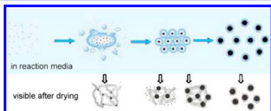
Figure 11. Schematic illustration of the formation of gold nanoparticles studied using AFM. Reprinted with permission from ref 65. Copyright 2011 Elsevier.
