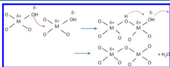
Figure 27. Formation of oxo bridges through a two step associative mechanism forming water.
