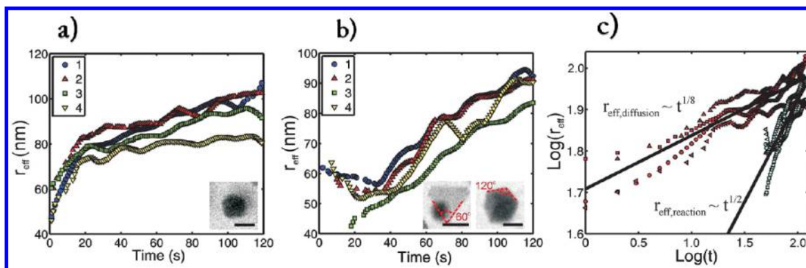
Figure 19. (a) Plot of the effective radius ( r_{\text{eff}} ) as a function of time for four individual nanocrystals. Inset is a higher magnification image showing the near spherical morphology of the resulting nanocrystal, the scale bar is 100 nm. (b) Plot of the effective radius as a function of time for four individual nanocrystals. Inset are higher magnification images showing the faceted morphology of the resulting nanocrystals; the scale bars are 100 nm. (c) Logarithmic relationship between the effective radius and time. The red data points correspond to panel a, while the blue correspond to panel b, the different markers correspond to the individual nanocrystals indicated in the legends of panels a and b. The black lines are the average power law fits for the four different nanocrystals, obtained by linear regression. A 10 point averaging filter was used on data a–c to reduce noise in the data. Adapted with permission from ref 78. Copyright 2012 American Chemical Society.
