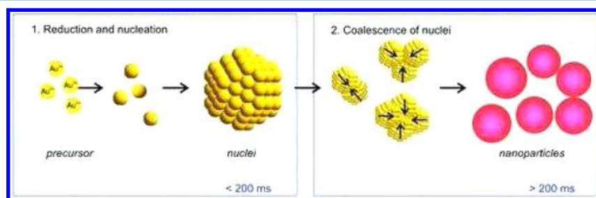
Figure 10. Schematic illustration of the formation of gold nanoparticles. Reprinted with permission from ref 63. Copyright 2010 American Chemical Society.
