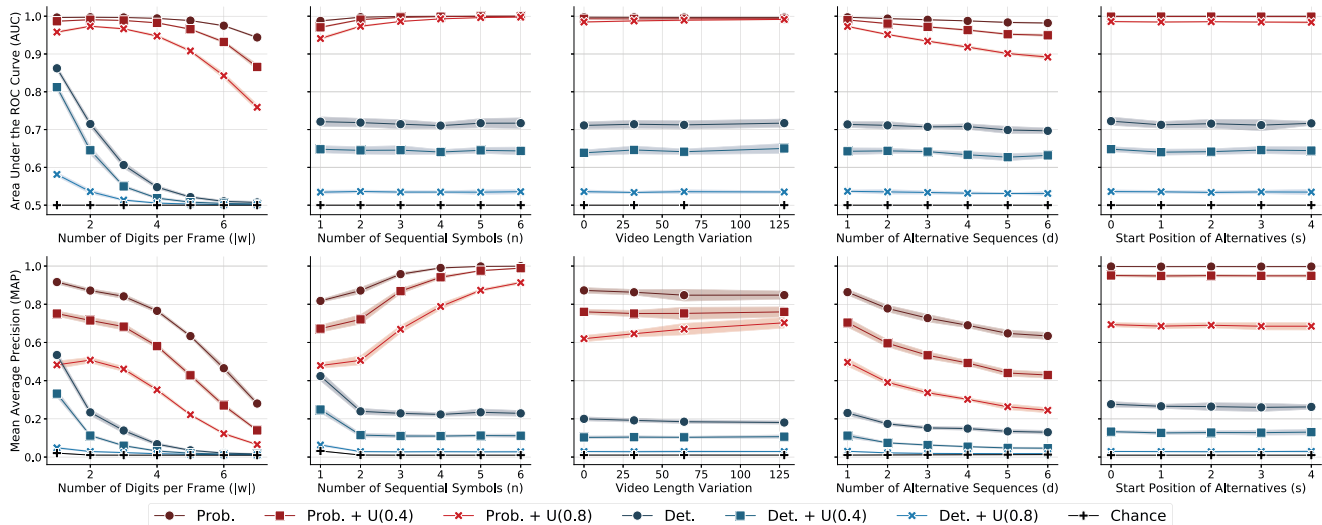
Figure 3. Plots of the performance, in terms of AUC and MAP, of the proposed methods on the generated synthetic dataset using primitive classifiers with different levels of noise as shown in Figure 2. The generated data consists of video clips depicting regular expressions parametrized according to Equation 7. We evaluate the proposed approaches according to the following data parameters: the number of digits that simultaneously appear in a frame |w| , the total number of different sequential symbols n , the variance in number of frames in the videos, the number of alternative sequences of symbols d , and the start position s of each alternative sequence in the pattern respectively.
