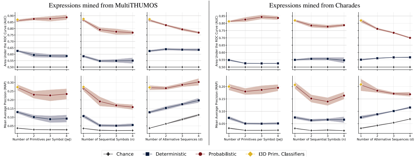
Figure 4. Comparison with standard action classification. Plots of the performance, in terms of AUC and MAP, of the proposed methods using the I3D model [1] as the primitive action classifier. We evaluate the models on collections of regular expressions of different complexity mined from the test videos of MultiTHUMOS and Charades datasets. These regular expressions follows the format defined in Equation 7 where all the variables are set to 1 with the exception of the one being evaluated. For instance, for the plot with variable number of sequential symbols ( n ) the expressions vary from (w_1^+) to (w_1^+ \succ \dots \succ w_4^+) . Differently from the other experiments, the symbols here denote any subset that contains the primitives.
