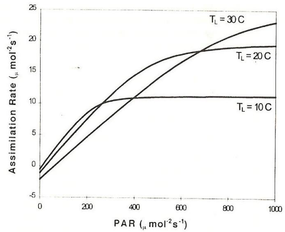
FIGURE 14.6. Photosynthesis as a function of PAR at three leaf temperatures.
