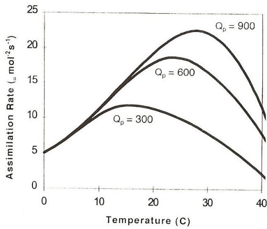
FIGURE 14.5. Temperature response of photosynthesis at three PAR levels for C_{ci} of 240 \mu\text{mol mol}^{-1} .
