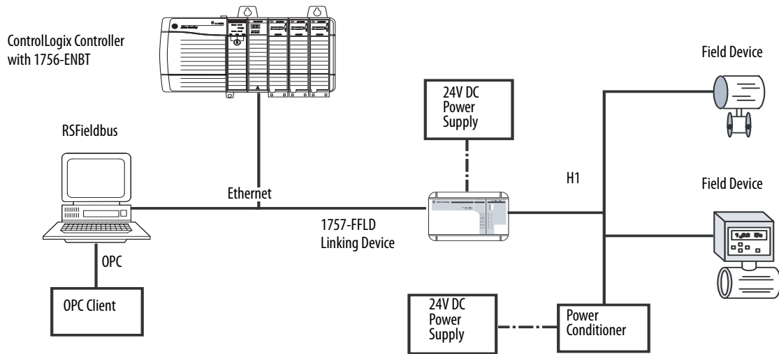
Figure 1 - Example Configuration - EtherNet/IP Network to FOUNDATION Fieldbus Network
